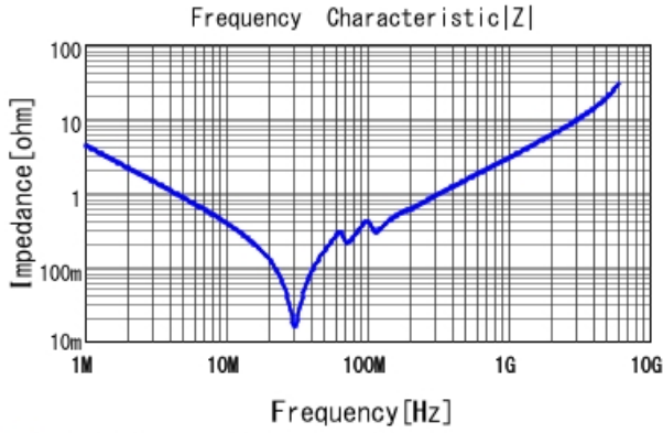
■ GRM3195C2A363JA01 |Z| DCOV, 25degC
