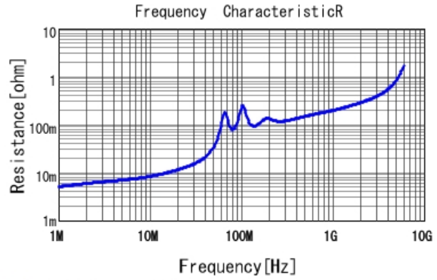
■ GRM3195C2A363JA01 R DCOV, 25degC
