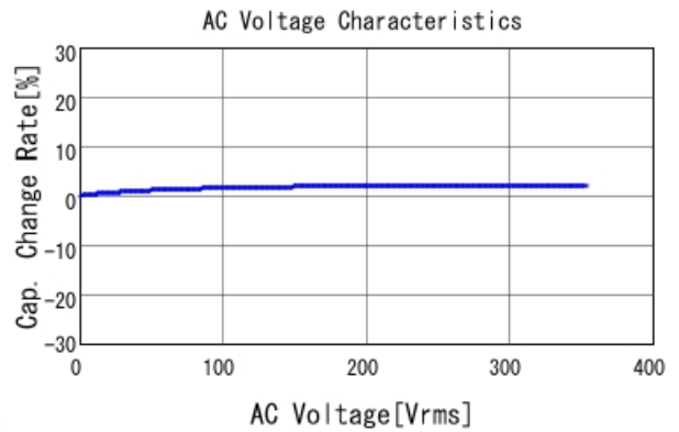
■ GRM31A7U3A120JW31 C-AC Voltage capchange, DCOV, 25.0d
