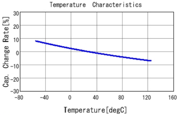
■ GRM31A7U3A120JW31 C-Temp. capchange, DCOV, AC1Vrms
