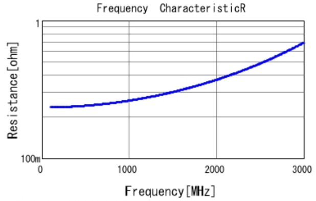
■ GRM31A7U3A120JW31 R DCOV, 25degC
