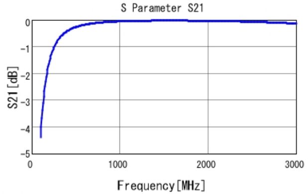
■ GRM31A7U3A120JW31 S21 DCOV, 25degC
