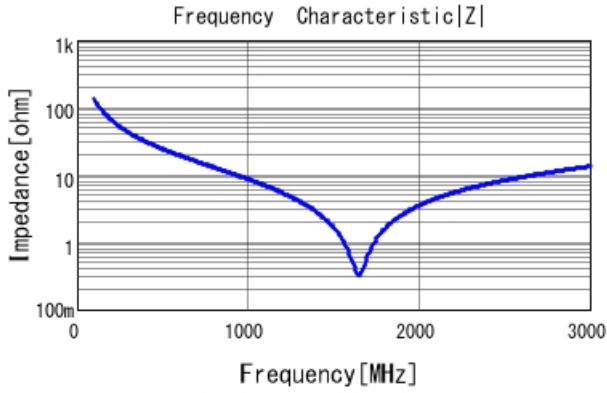
■ GRM31A7U3A120JW31 |Z| DCOV, 25degC
