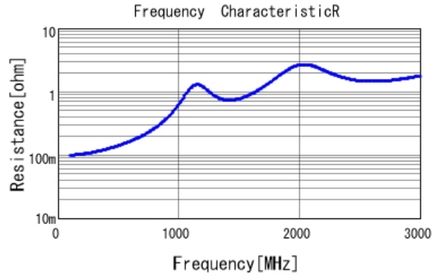
■ GRM31A7U3A181JW31 R DCOV, 25degC
