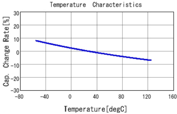
■ GRM31A7U3A181JW31 C-Temp. capchange, DCOV, AC1Vrms
