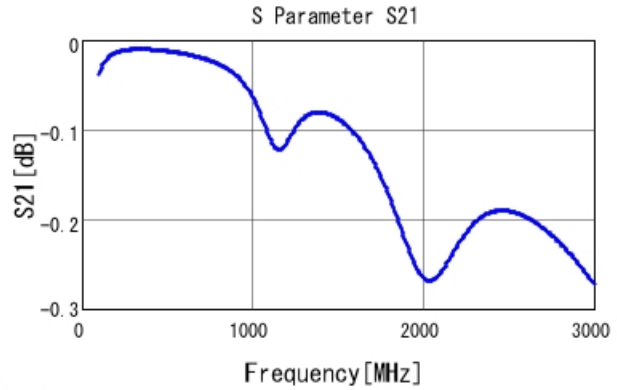
■ GRM31A7U3A181JW31 S21 DCOV, 25degC
