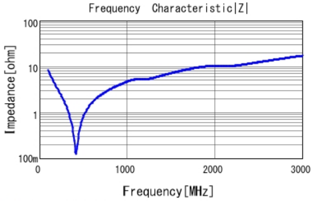
■ GRM31A7U3A181JW31 |Z| DCOV, 25degC
