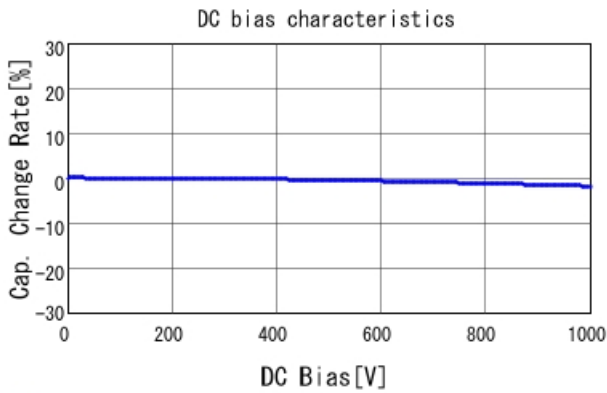
■ GRM31A7U3A820JW31 C-DC bias capchange, 25.0degC, AC1V
