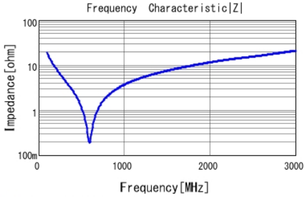
■ GRM31A7U3A820JW31 |Z| DCOV, 25degC
