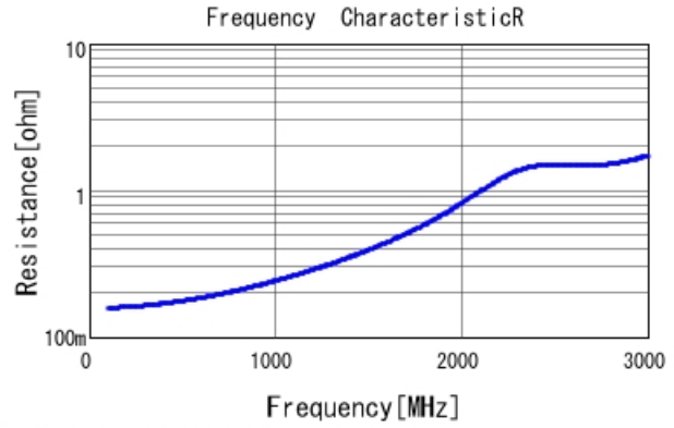
■ GRM31A7U3A820JW31 R DCOV, 25degC
