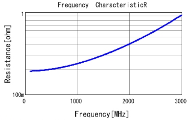
■ GRM31A7U3D120JW31 R DCOV, 25degC
