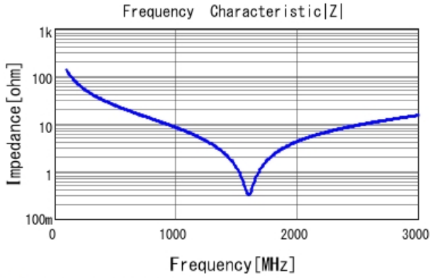
■ GRM31A7U3D120JW31 |Z| DCOV, 25degC
