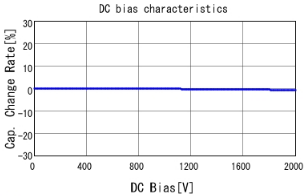
■ GRM31A7U3D120JW31 C-DC bias capchange, 25.0degC, AC1V
