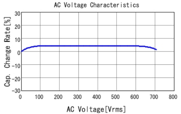
■ GRM31A7U3D120JW31 C-AC Voltage capchange, DCOV, 25.0d
