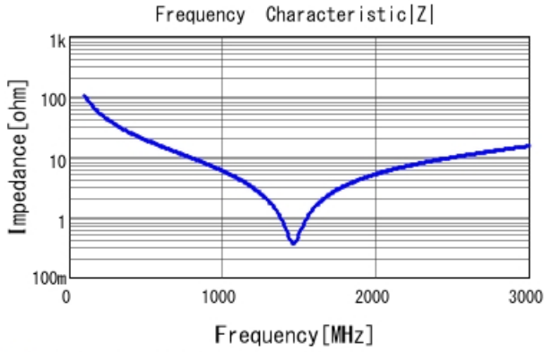
■ GRM31A7U3D150JW31 |Z| DC0V, 25degC
