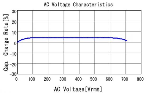
■ GRM31A7U3D150JW31 C-AC Voltage capchange, DC0V, 25.0d
