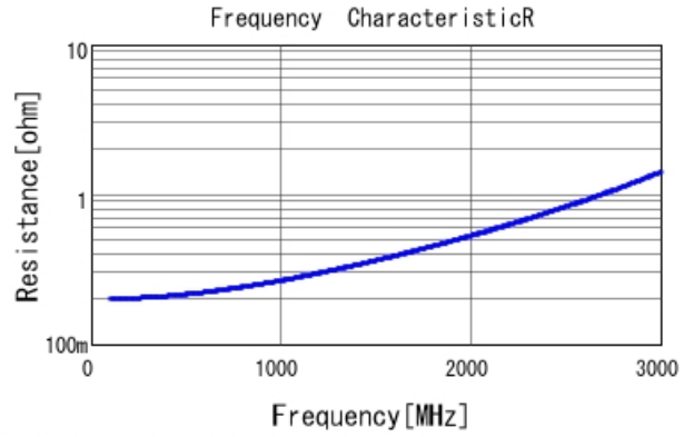
■ GRM31A7U3D150JW31 R DC0V, 25degC
