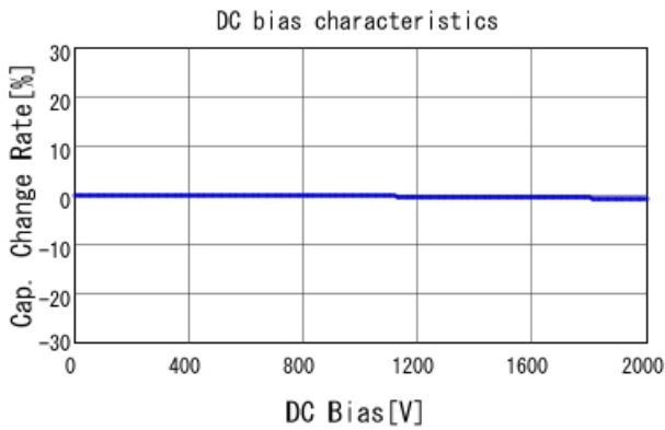
■ GRM31A7U3D150JW31 C-DC bias capchange, 25.0degC, AC1V
