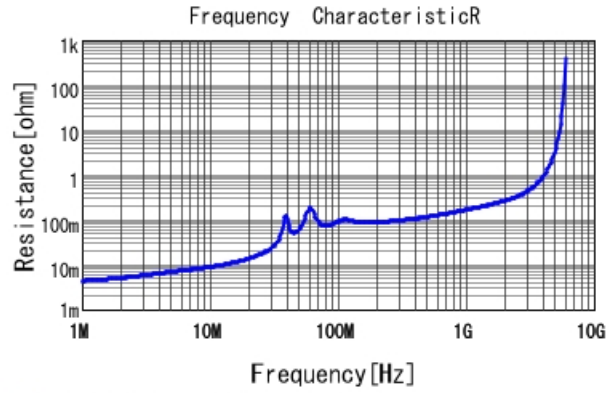
■ GRM31C5C2A753JA01 R DCOV, 25degC
