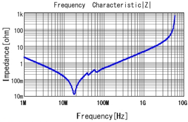
■ GRM31C5C2A753JA01 |Z| DCOV, 25degC
