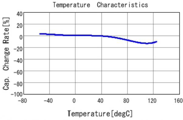
■ GRM55DR72E334KW01 C-Temp. capchange, DCOV, AC1Vrms
