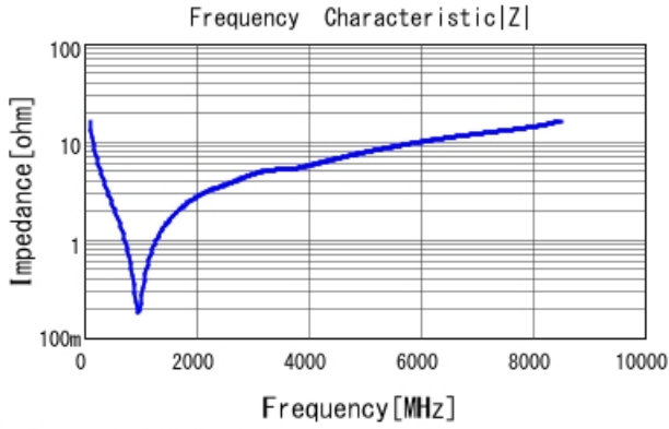
■ GRT0335C1H101FA02 |Z| DC0V, 25degC
