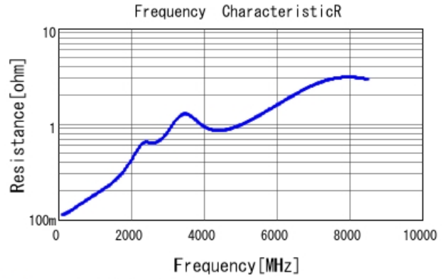
■ GRT0335C1H101FA02 R DC0V, 25degC
