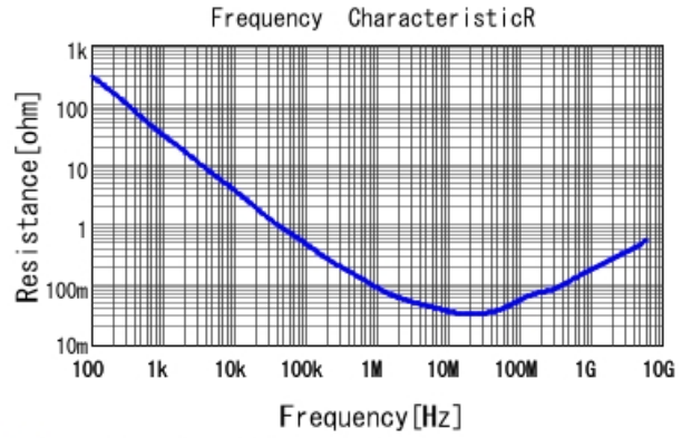
GRT033R61E104KE01 R DC0V, 25degC
