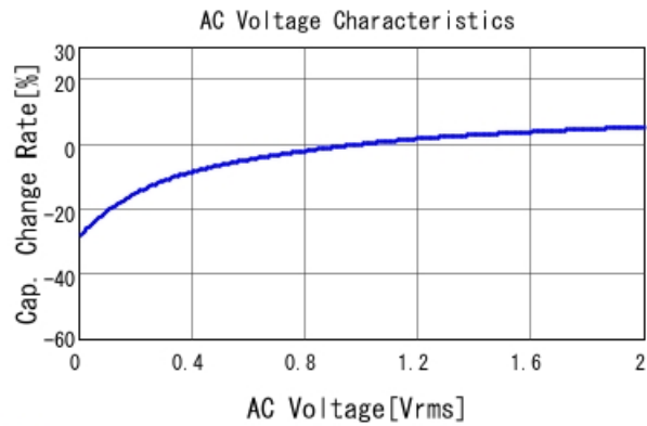
GRT033R61E104KE01 C-AC Voltage capchange, DC0V, 25.0d
