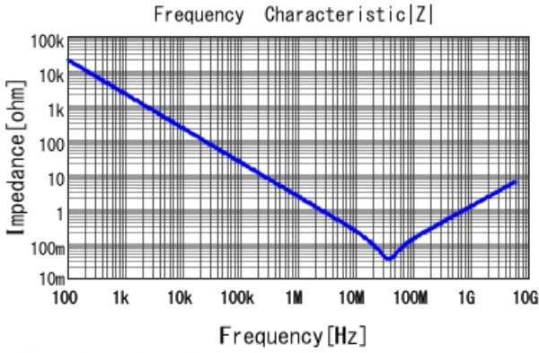
GRT033R61E104KE01 |Z| DC0V, 25degC
