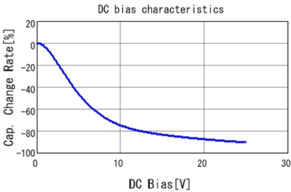
GRT033R61E104KE01 C-DC bias capchange, 25.0degC, AC1V
