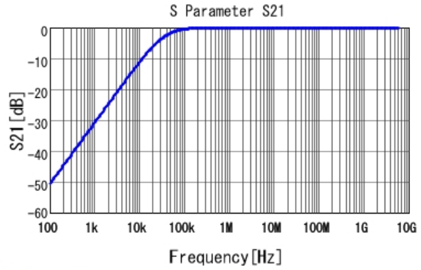
■ GRT155R71H473KE01 S21 DCOV, 25degC
