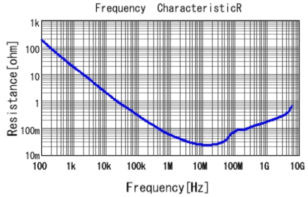
GRT155R71H473KE01 R DC0V, 25degC
