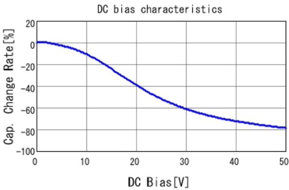
GRT155R71H473KE01 C-DC bias capchange, 25.0degC, AC1.
