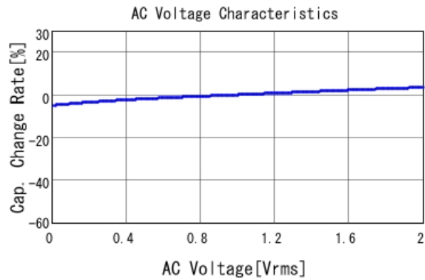
GRT155R71H473KE01 C-AC Voltage capchange, DC0V, 25.0d
