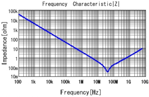
GRT155R71H473KE01 |Z| DC0V, 25degC
