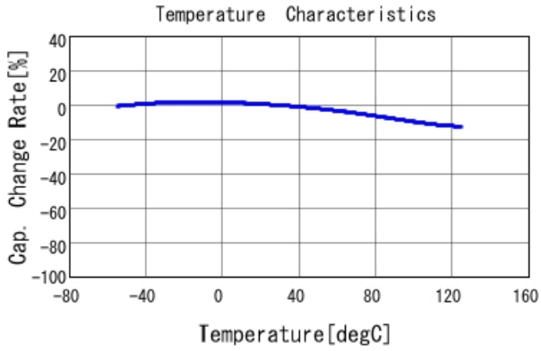
■ GRT155R71H473KE01 C-Temp. capchange, DCO. 0V, AC1.0V rm
