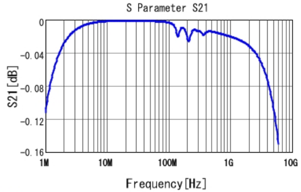
■ GRT1885C1H103JA02 S21 DCOV, 25degC
