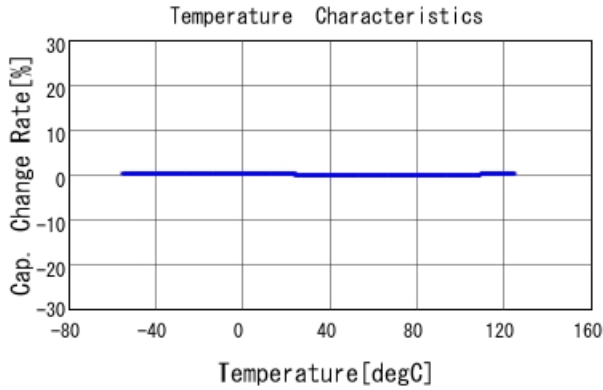
■ GRT1885C1H103JA02 C-Temp. capchange, DCOV, AC1Vrms
