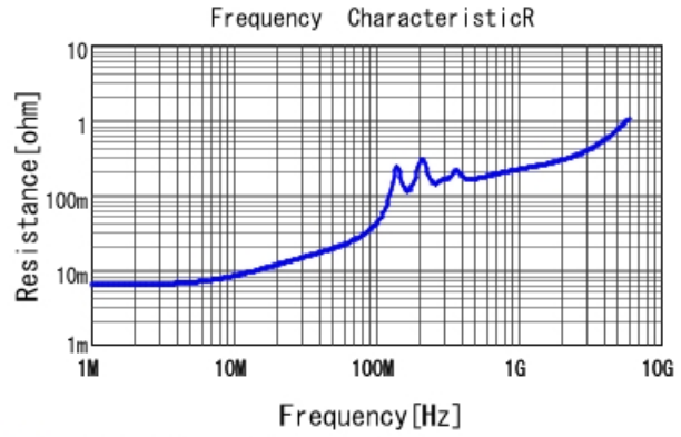
■ GRT1885C1H103JA02 R DCOV, 25degC
