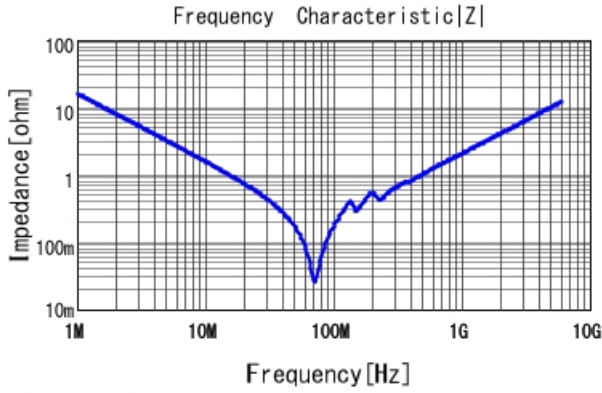
■ GRT1885C1H103JA02 |Z| DCOV, 25degC
