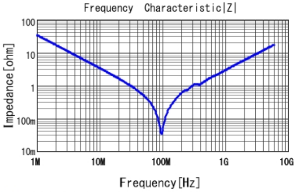
■ GRT1885C1H472JA02 |Z| DCOV, 25degC
