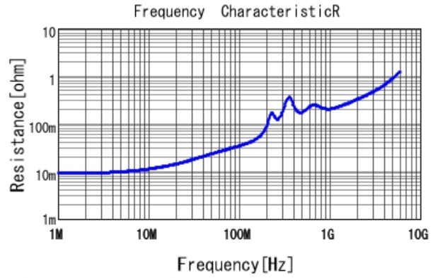
■ GRT1885C1H472JA02 R DCOV, 25degC
