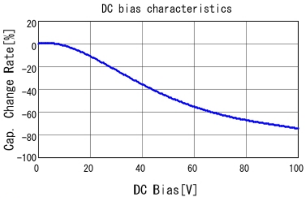
■ KCM55QR72A685KH01 C-DC bias capchange, 25.0degC, AC1V
