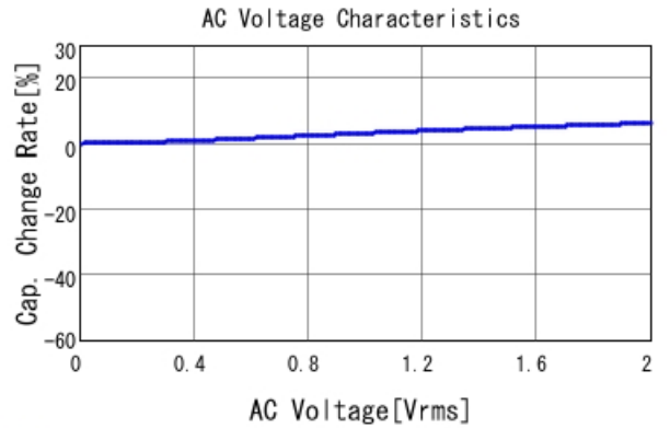
■ KCM55QR72A685KH01 C-AC Voltage capchange, DCOV, 25.0d
