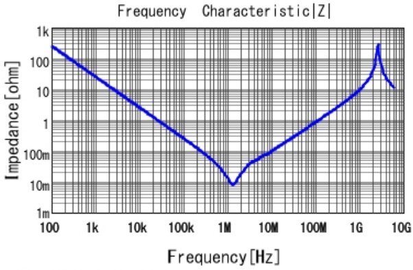
■ KCM55QR72A685KH01 |Z| DCOV, 25degC
