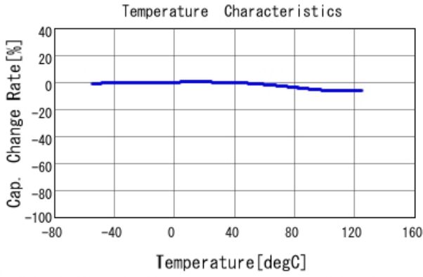
■ KCM55QR72A685KH01 C-Temp. capchange, DCOV, AC1Vrms
