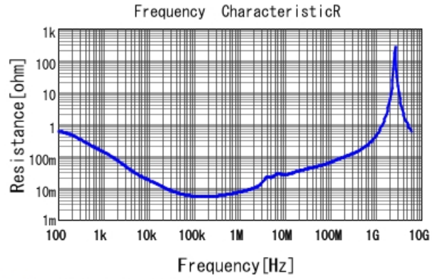
■ KCM55QR72A685KH01 R DCOV, 25degC
