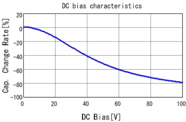
■ GCJ31CR72A105KA01 C-DC bias capchange, 25.0degC, AC1.
