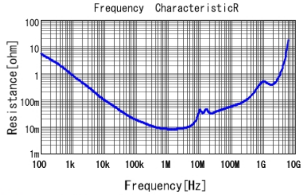
■ GCJ31CR72A105KA01 R DC0V, 25degC
