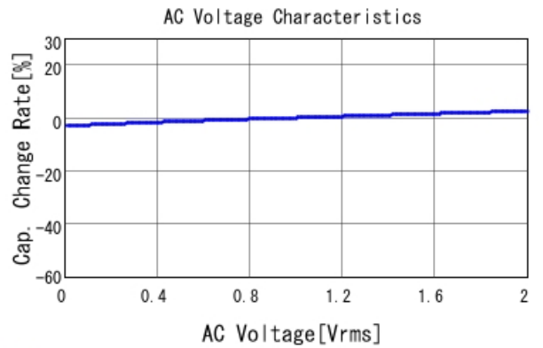
■ GCJ31CR72A105KA01 C-AC Voltage capchange, DC0V, 25.0d
