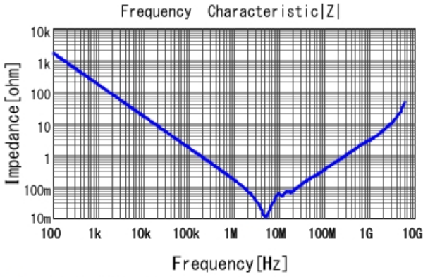
■ GCJ31CR72A105KA01 |Z| DC0V, 25degC
