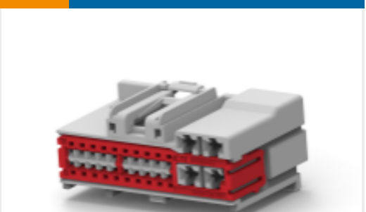
TE Part #1-2236269-2 24POS, MIXED,REC HSG, 20GENYMCP,ASSY,CODB
