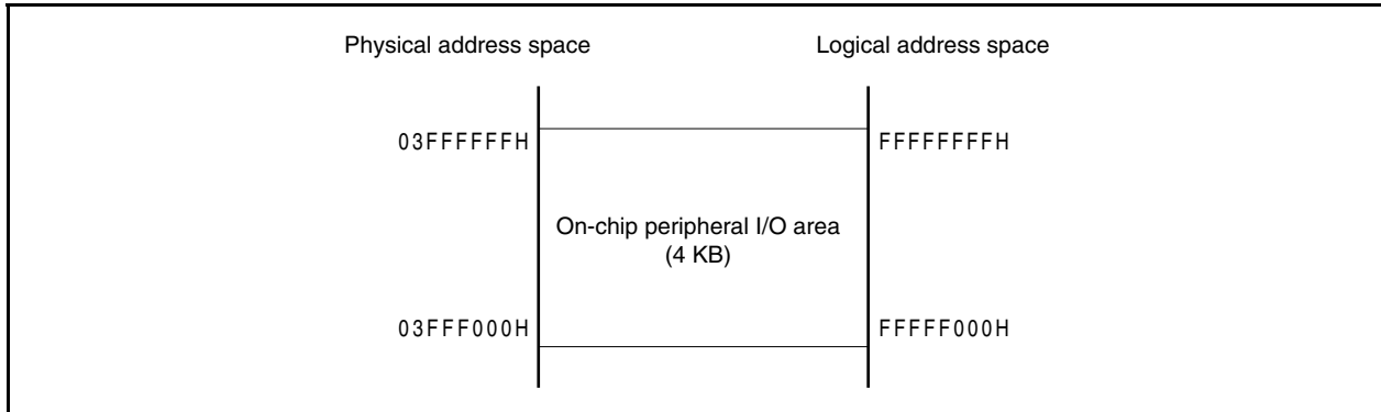
Figure 3-13. On-Chip Peripheral I/O Area
