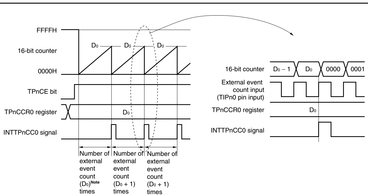
Figure 7-14. Basic Timing in External Event Count Mode
