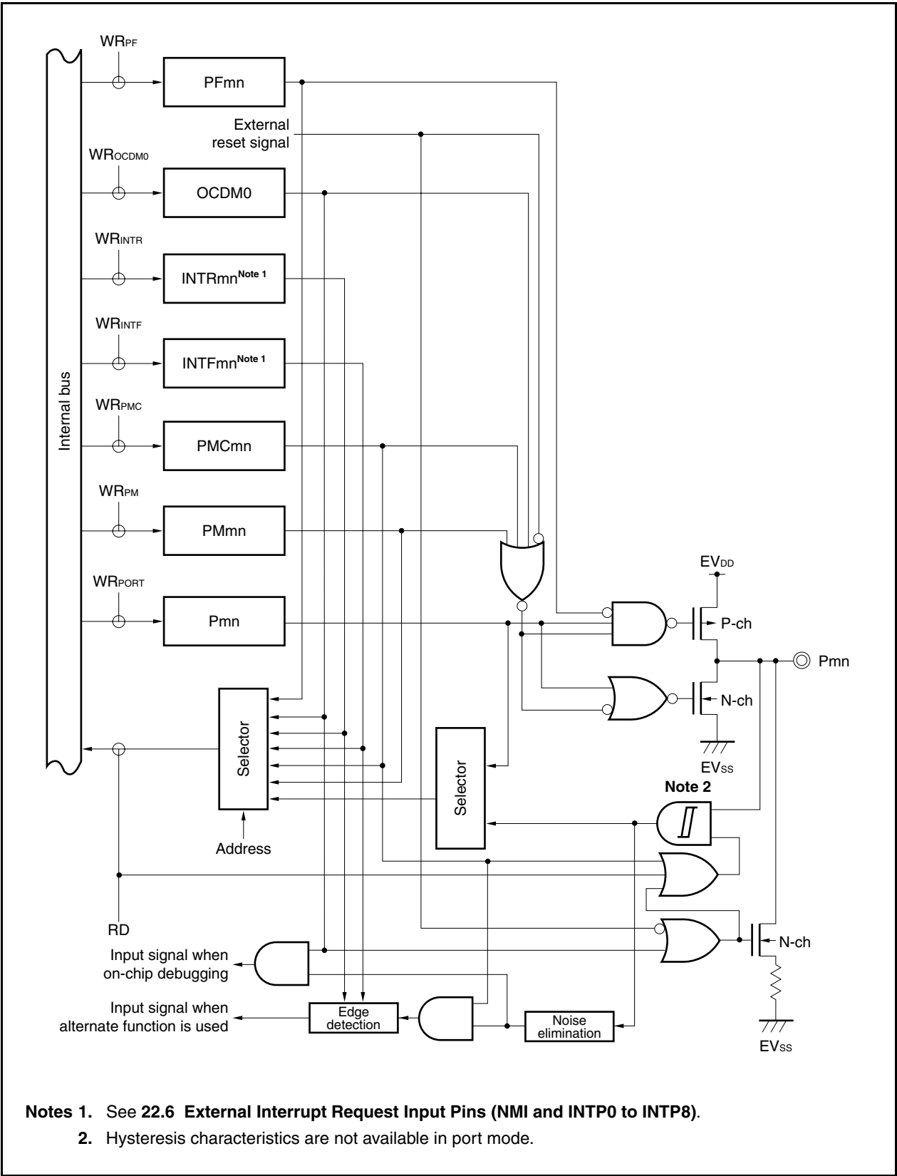
Figure 4-40. Block Diagram of Type AA-1
