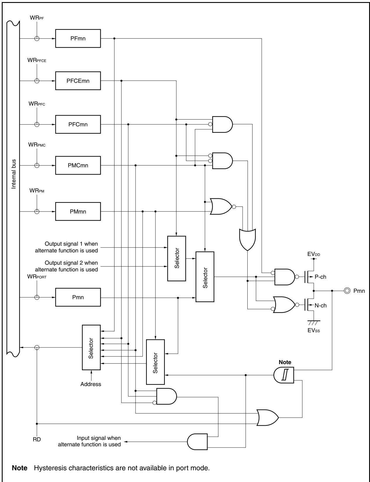
Figure 4-36. Block Diagram of Type U-12
