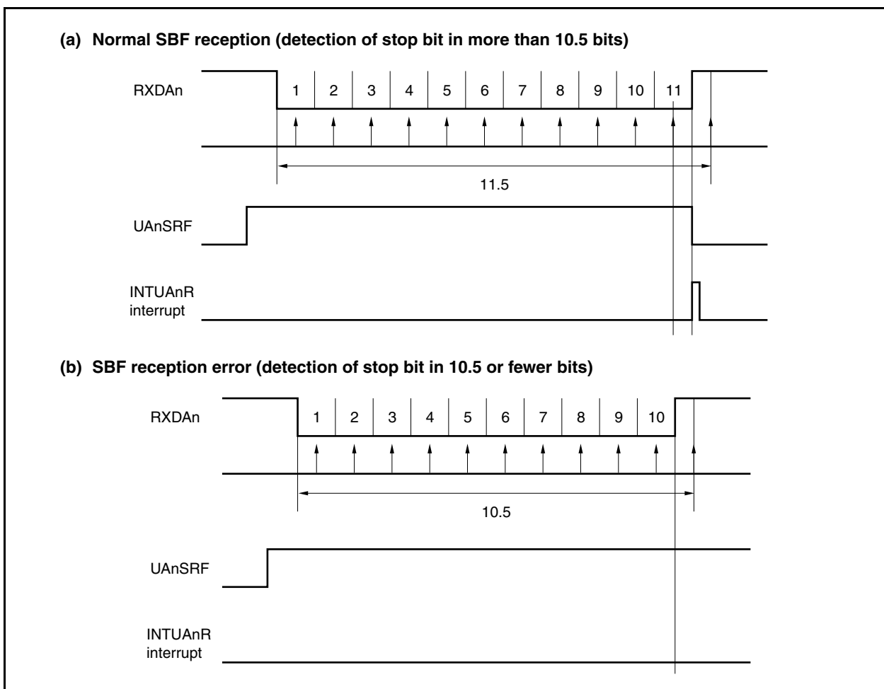
Figure 15-9. SBF Reception
