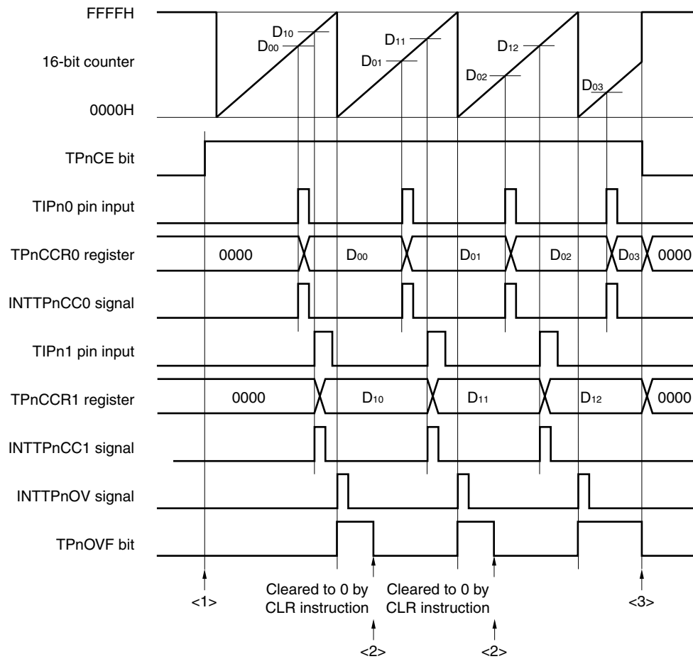
Figure 7-37. Software Processing Flow in Free-Running Timer Mode (Capture Function) (1/2)
