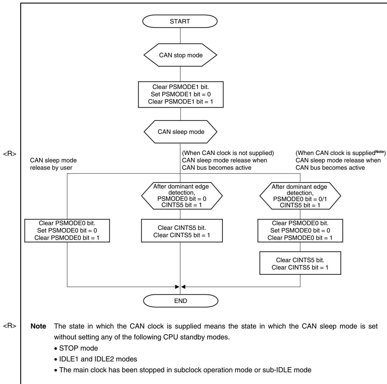
Figure 19-53. Clear CAN Sleep/Stop Mode
