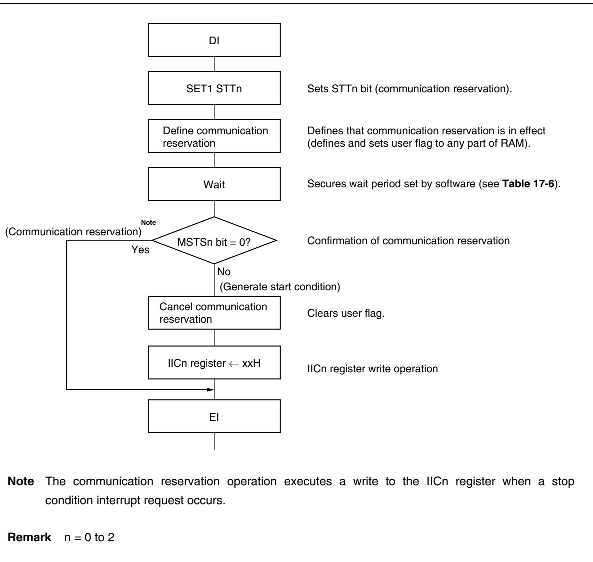
Figure 17-17. Communication Reservation Flowchart
