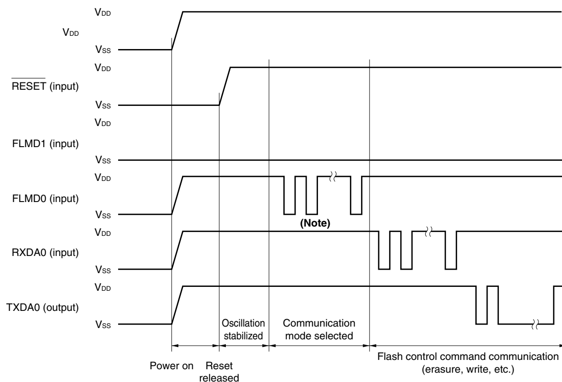
Figure 30-8. Selection of Communication Mode
