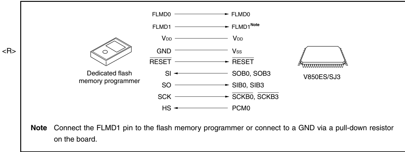
Figure 30-5. Communication with Dedicated Flash Memory Programmer (CSIB0 + HS, CSIB3 + HS)
