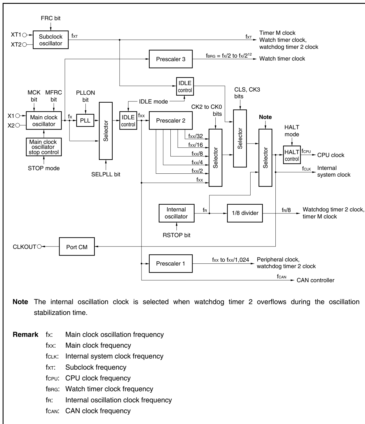
Figure 6-1. Clock Generator
