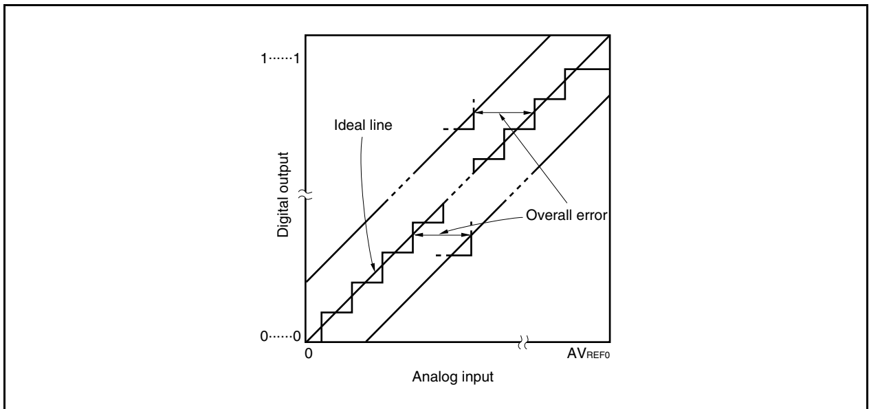
Figure 13-16. Overall Error
