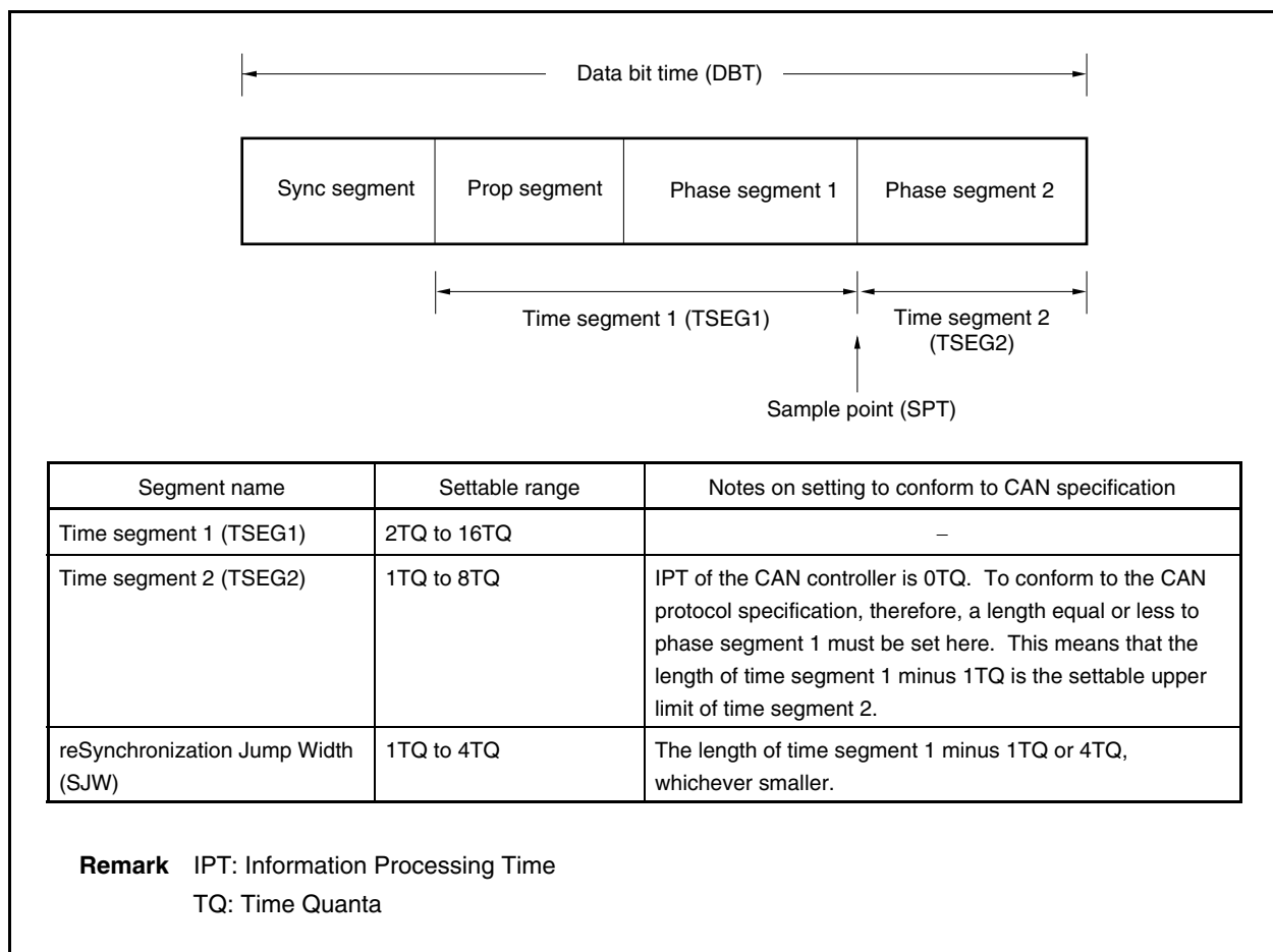
Figure 19-18. Segment Setting
