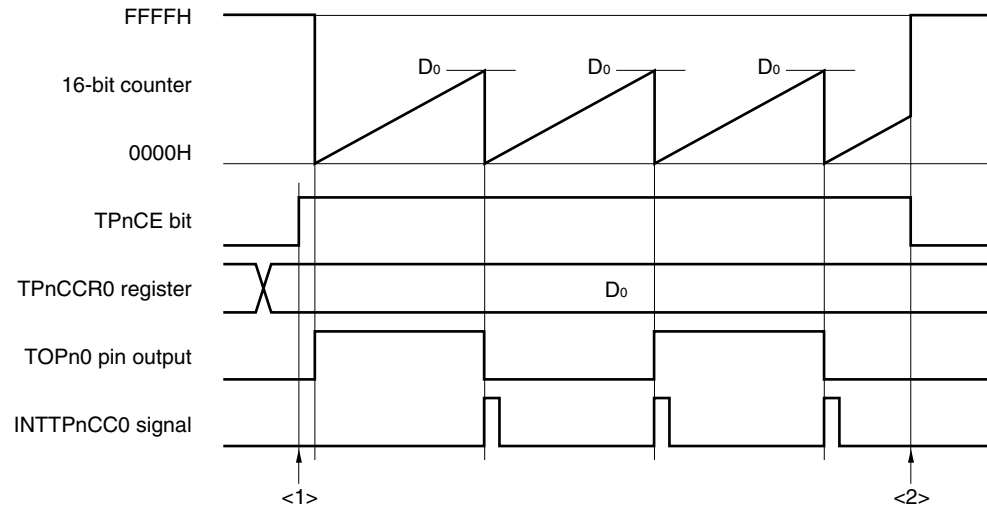
Figure 7-9. Software Processing Flow in Interval Timer Mode
