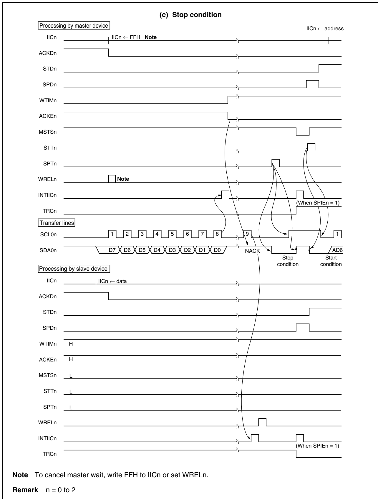
Figure 17-24. Example of Slave to Master Communication (When 8- → 9-Clock Wait for Master and 9-Clock Wait for Slave Are Selected) (3/3)
