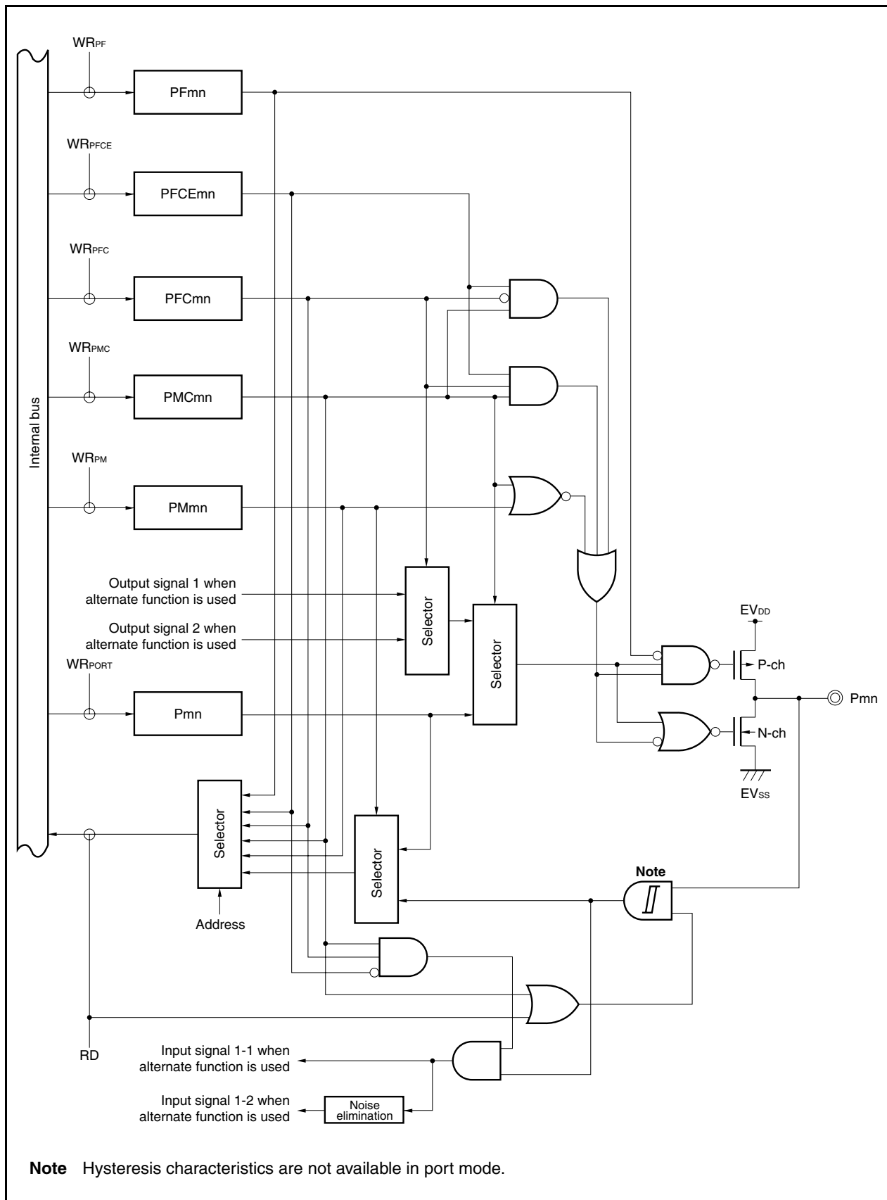
Figure 4-29. Block Diagram of Type U-5
