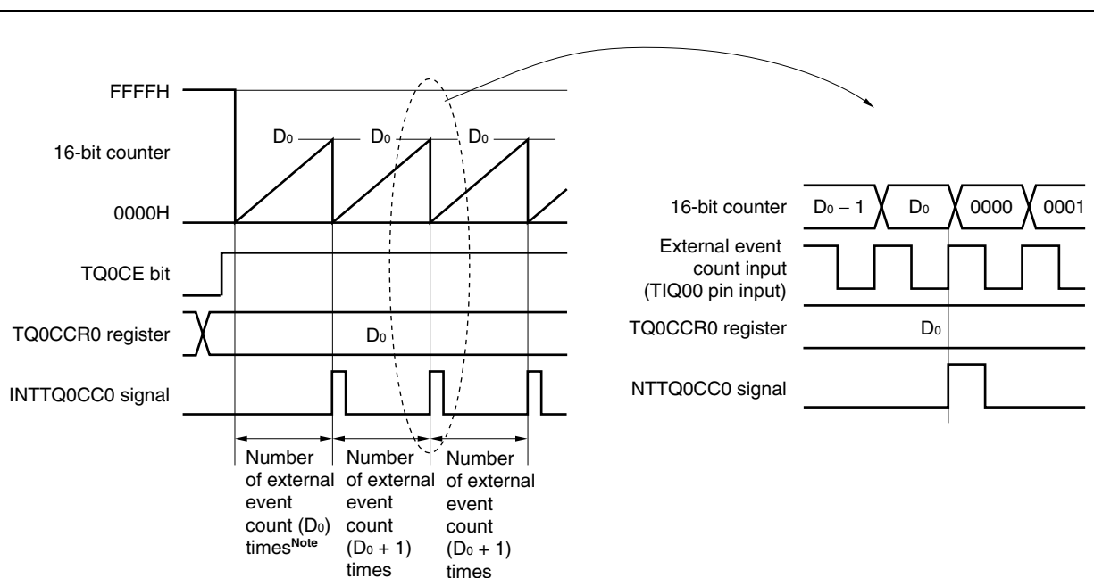
Figure 8-14. Basic Timing in External Event Count Mode
