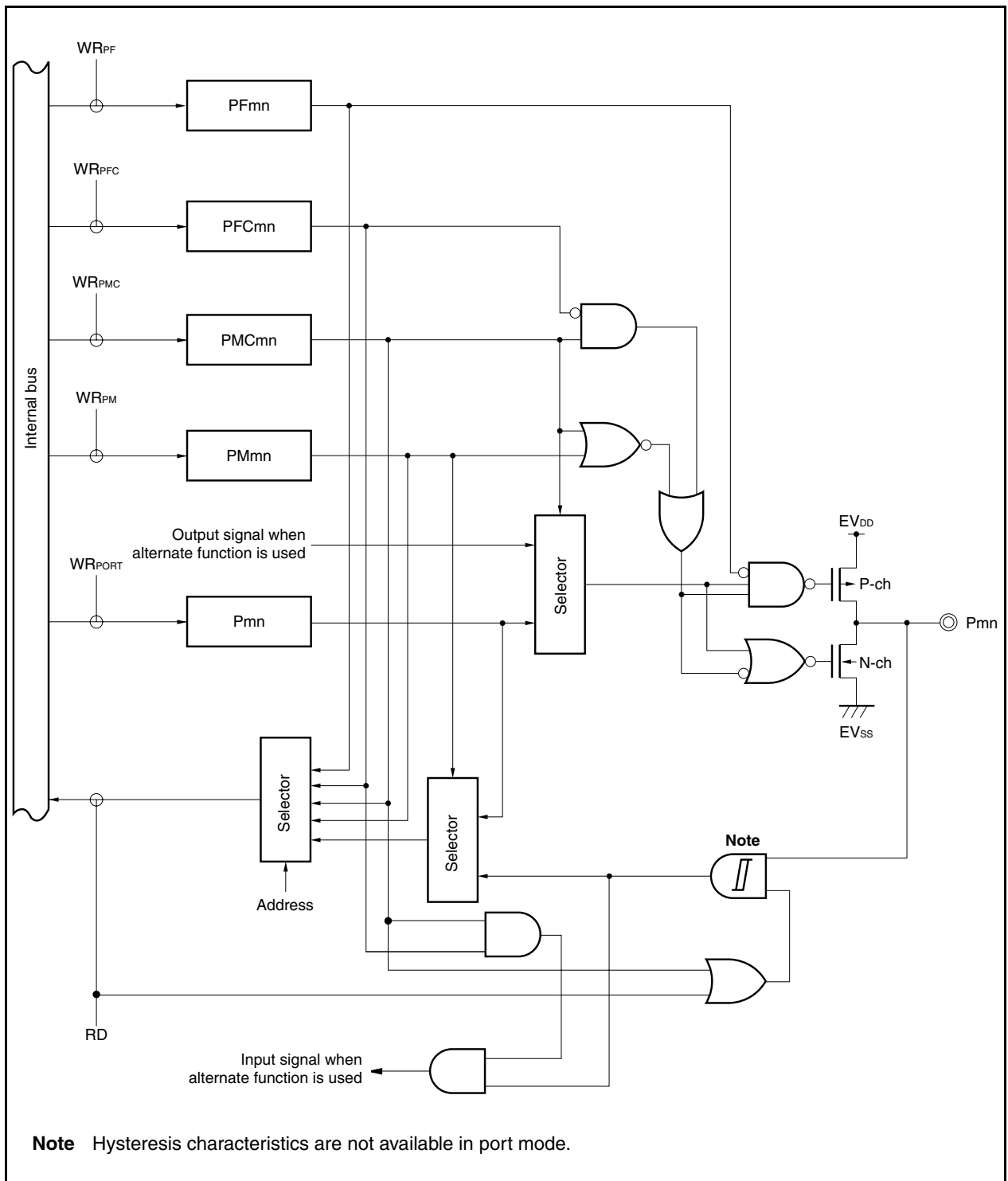
Figure 4-14. Block Diagram of Type G-2
