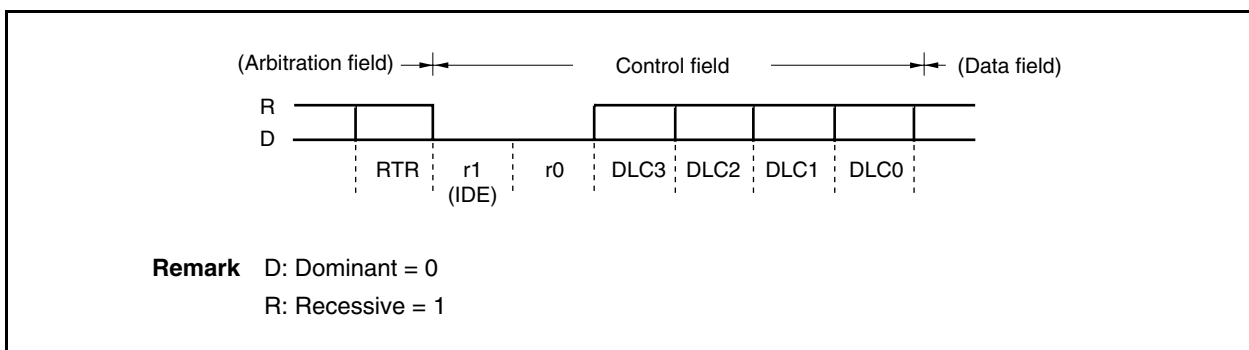
Figure 19-8. Control Field
