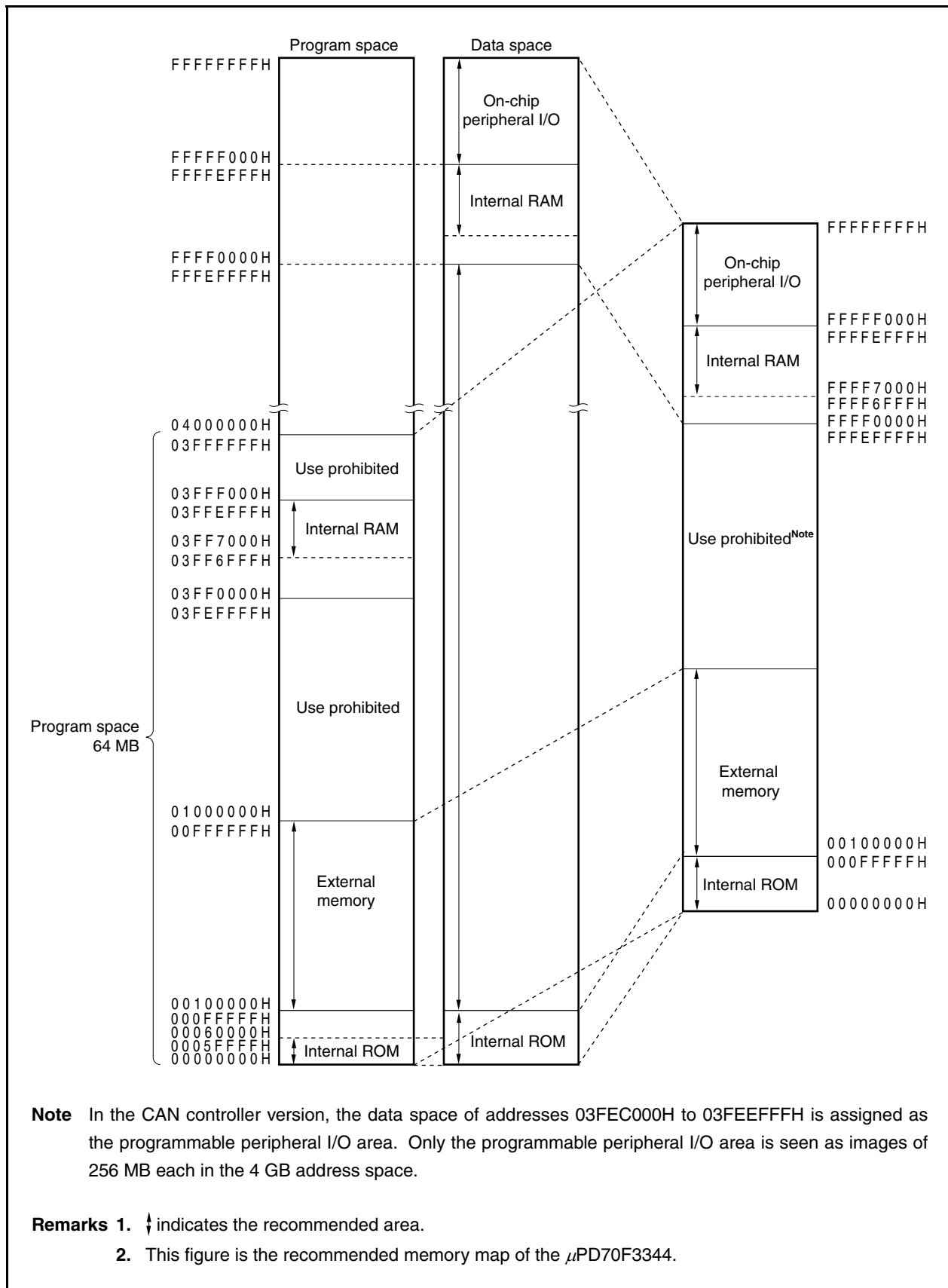
Figure 3-15. Recommended Memory Map
