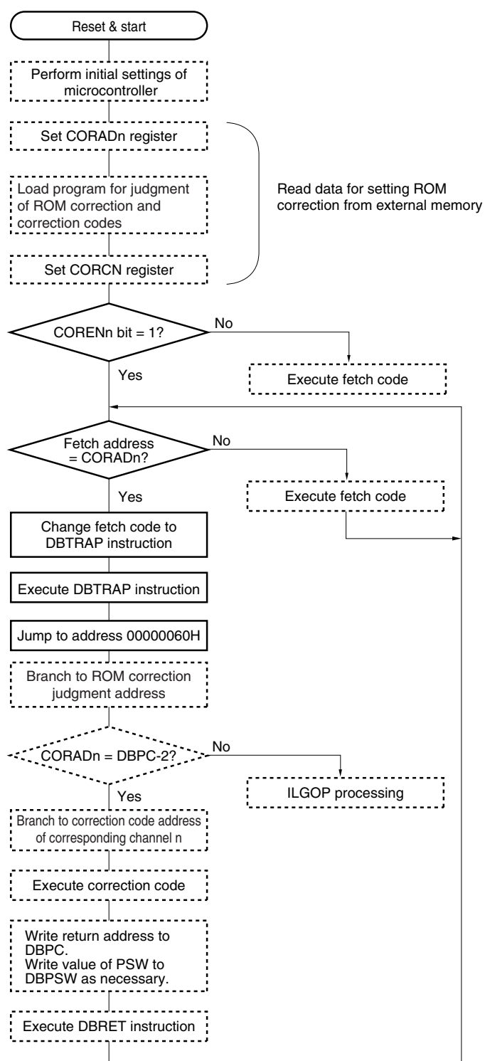
Figure 29-2. ROM Correction Operation and Program Flow
