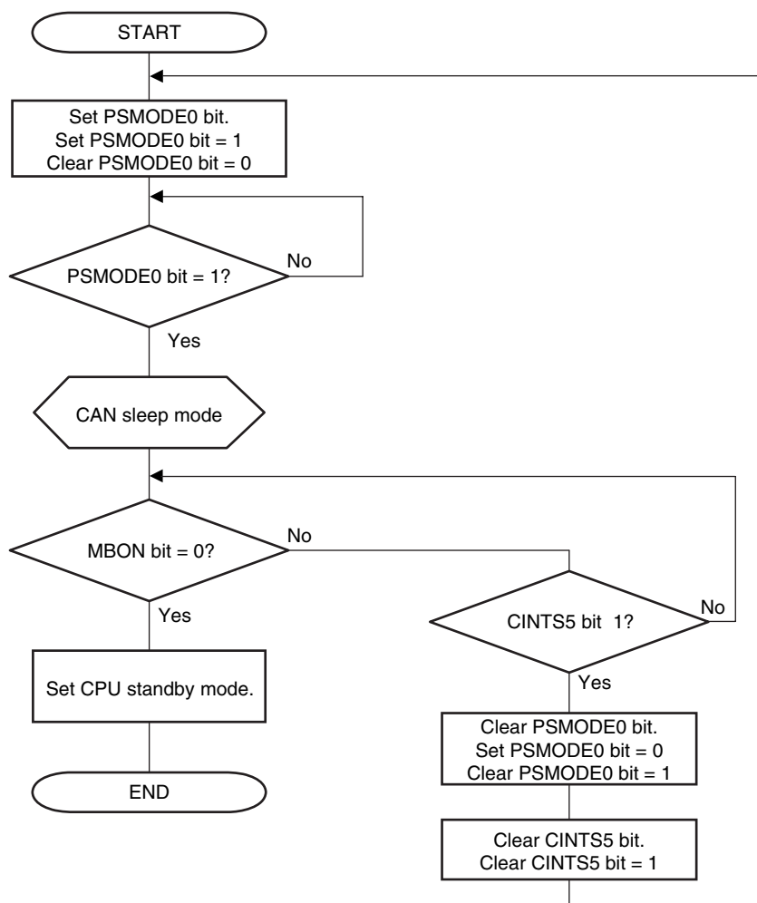
Figure 19-59. Setting CPU Standby (from CAN Sleep Mode)
