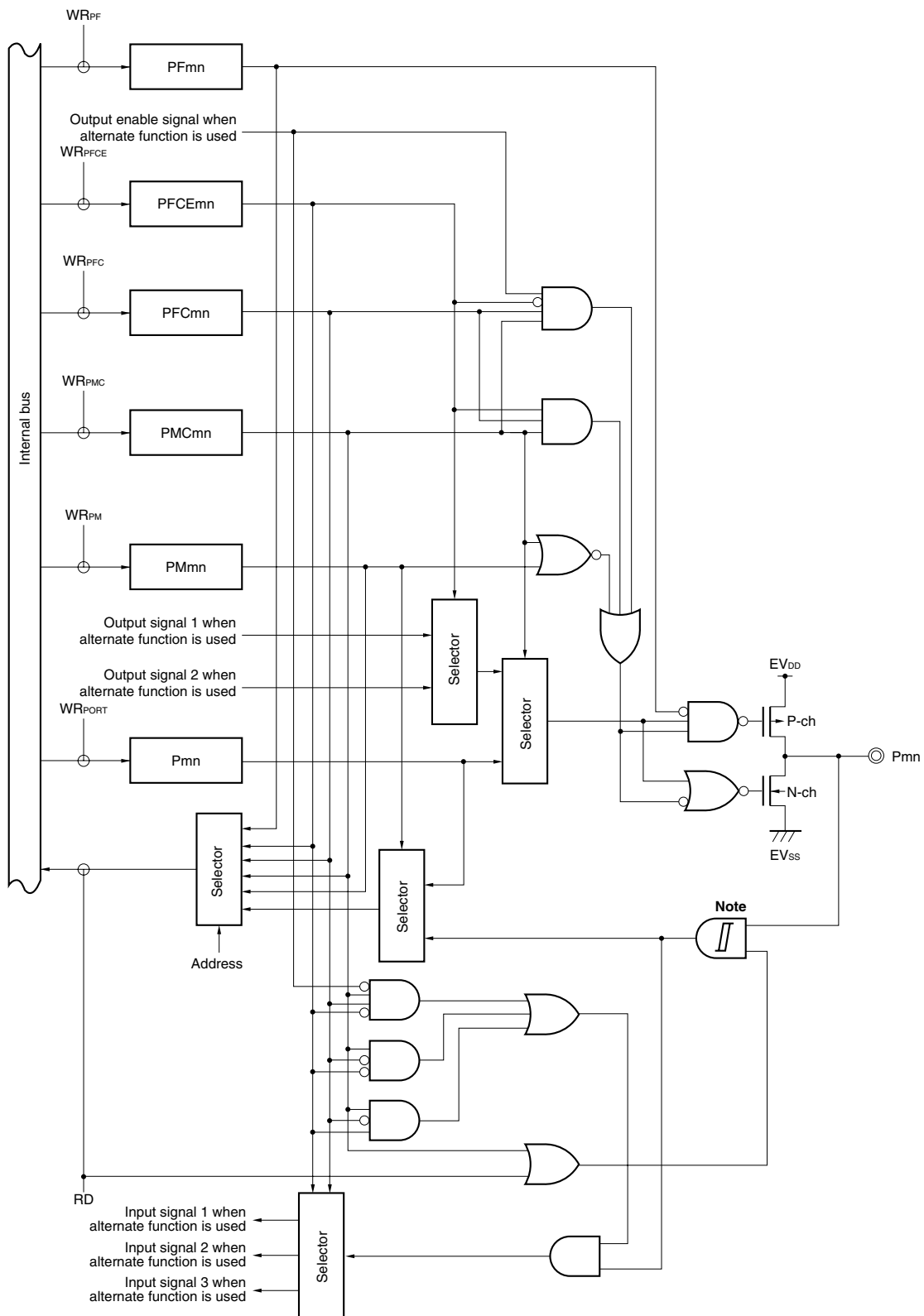
Figure 4-25. Block Diagram of Type U-1
