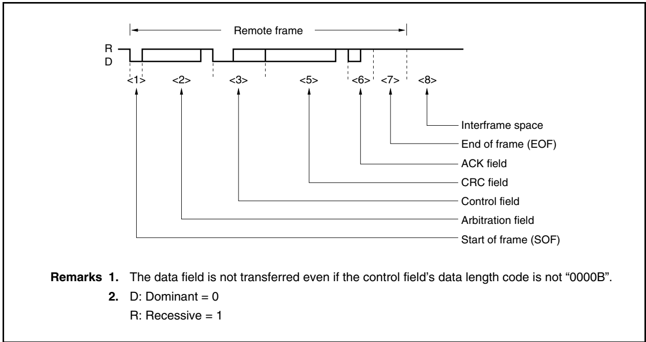
Figure 19-4. Remote Frame
