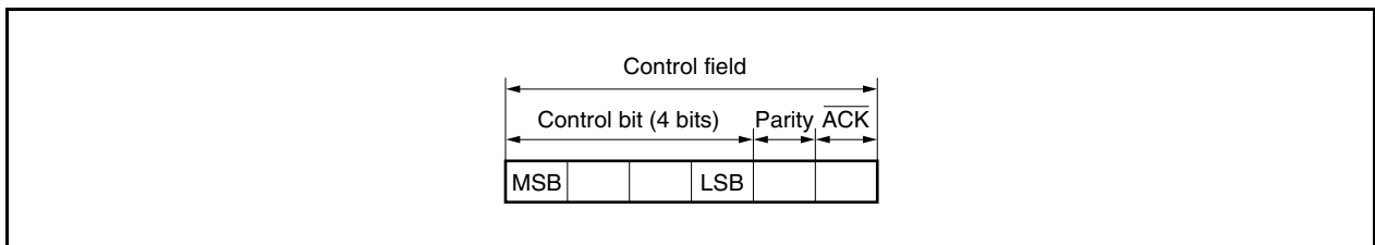
Figure 18-4. Control Field
