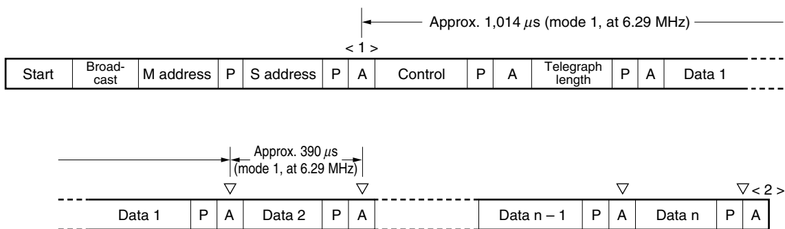
Figure 18-27. Master Reception
