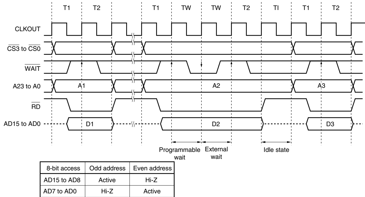
Figure 5-9. Separate Bus Read Timing (Bus Size: 16 Bits, 16-Bit Access)
