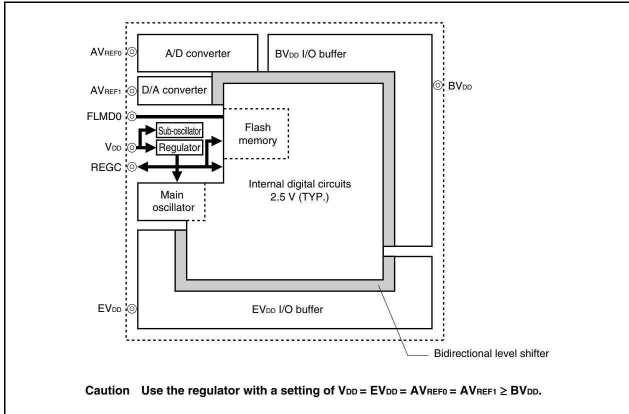
Figure 28-1. Regulator
