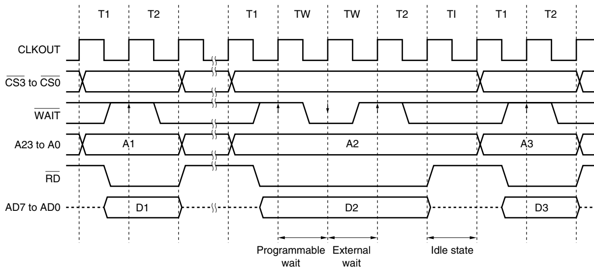
Figure 5-10. Separate Bus Read Timing (Bus Size: 8 Bits)
