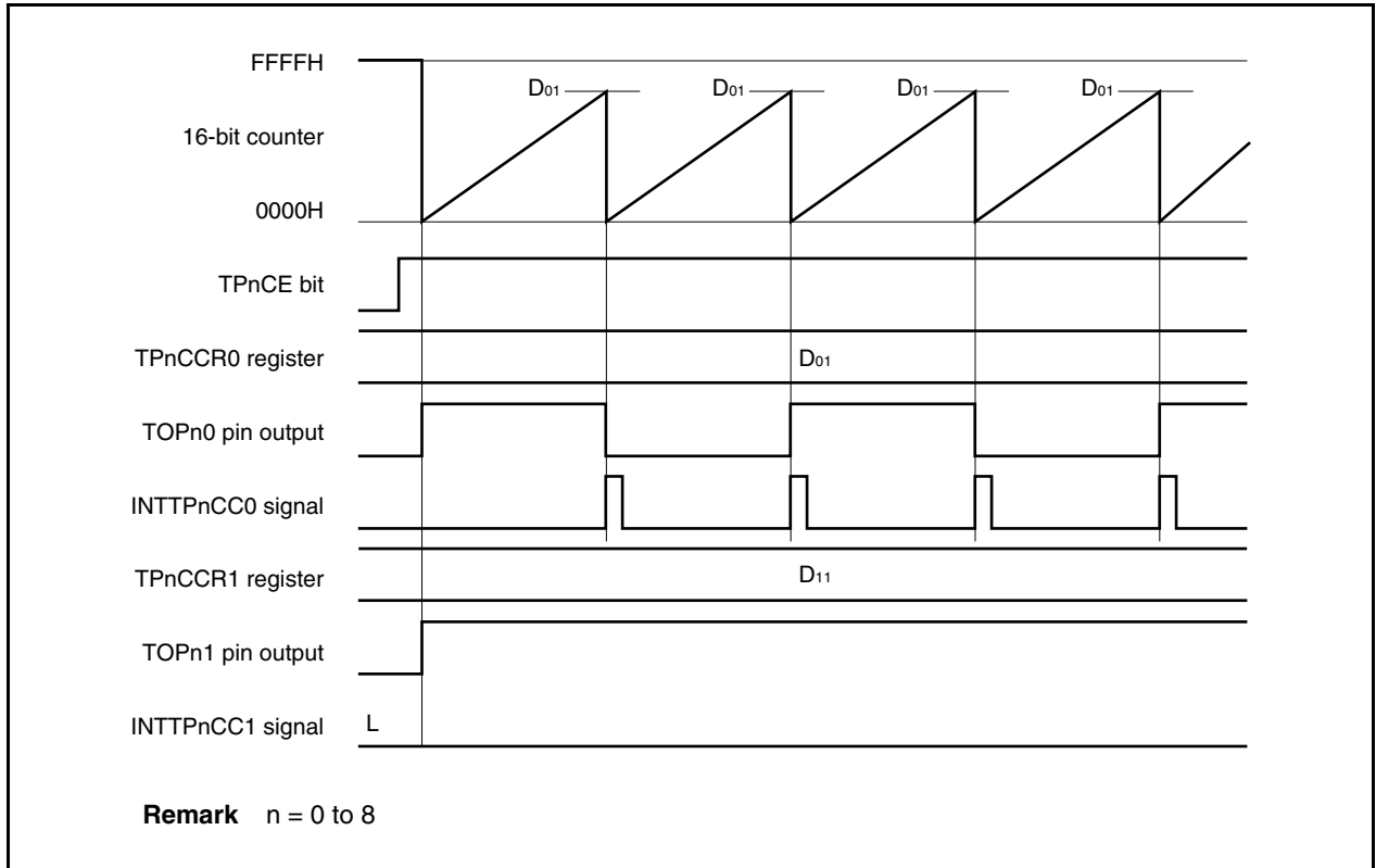
Figure 7-12. Timing Chart When D_{01} < D_{11}
