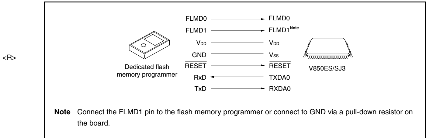
Figure 30-3. Communication with Dedicated Flash Memory Programmer (UARTA0)
