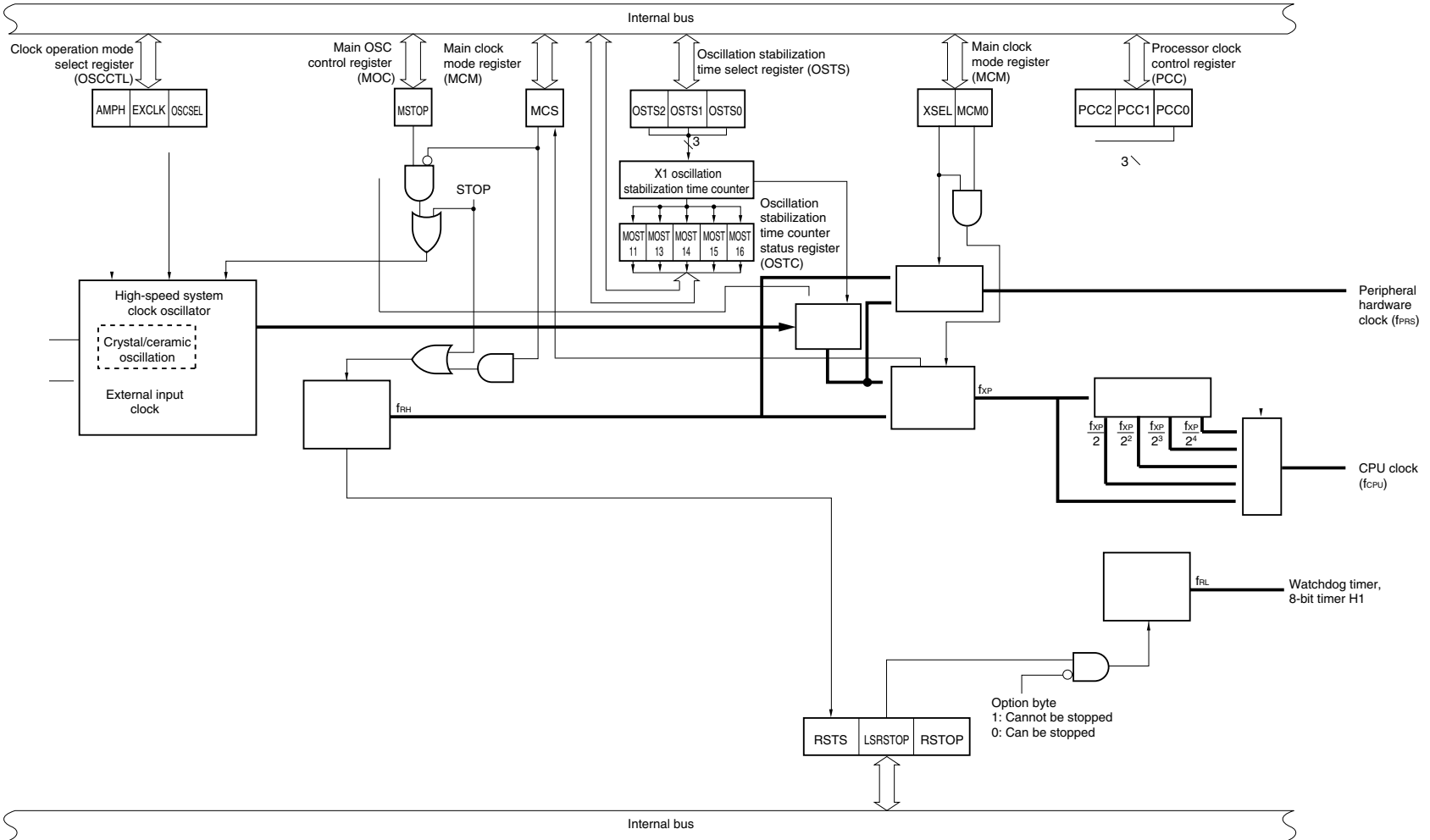
Figure 5-1. Block Diagram of Clock Generator
