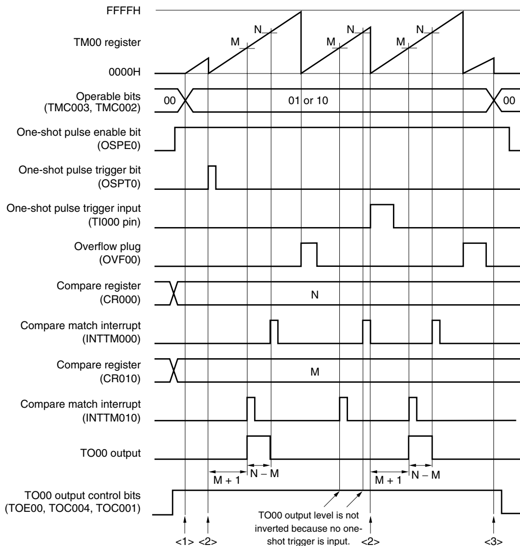
<R> Figure 6-45. Example of Software Processing for One-Shot Pulse Output Operation (1/2)
