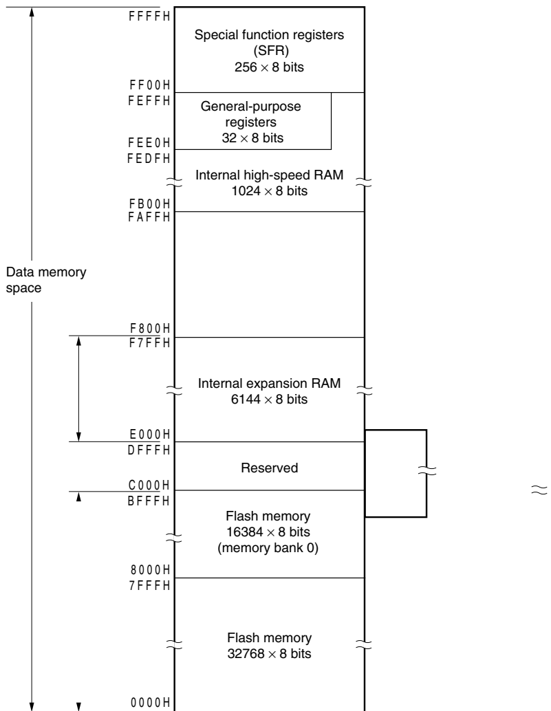
Figure 3-4. Memory Map ( \mu PD78F0547)
