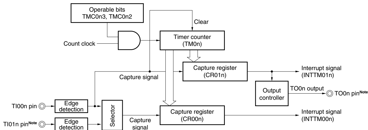
<R> Figure 7-33. Block Diagram of Clear & Start Mode Entered by TI00n Pin Valid Edge Input (CR00n: Capture Register, CR01n: Capture Register)
