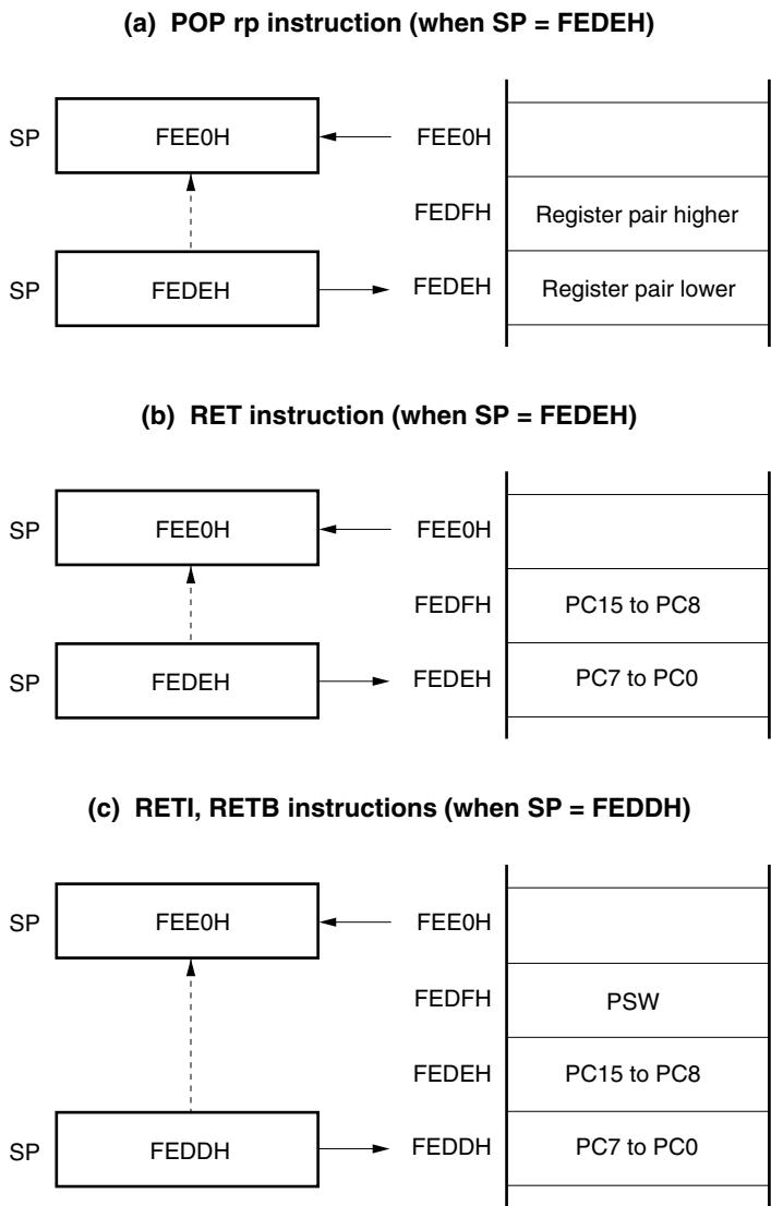
Figure 3-14. Data to Be Restored from Stack Memory
