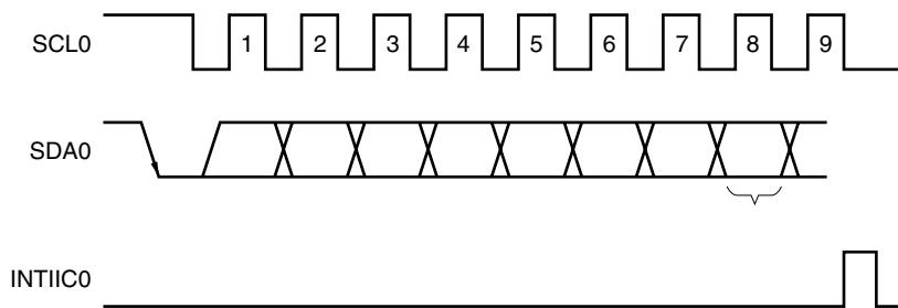
Figure 18-15. Transfer Direction Specification
