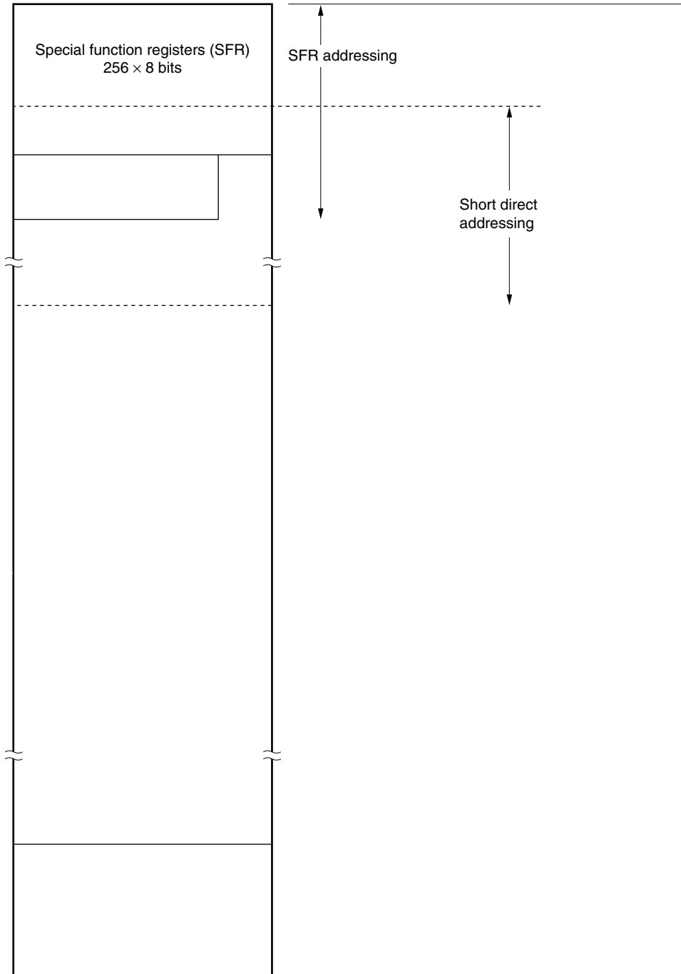
Figure 3-6. Correspondence Between Data Memory and Addressing ( \mu PD78F0544)
