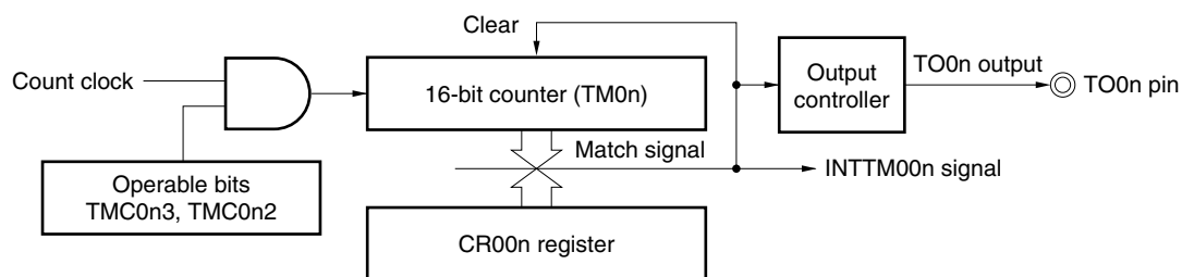
<R> Figure 7-20. Block Diagram of Square-Wave Output Operation
