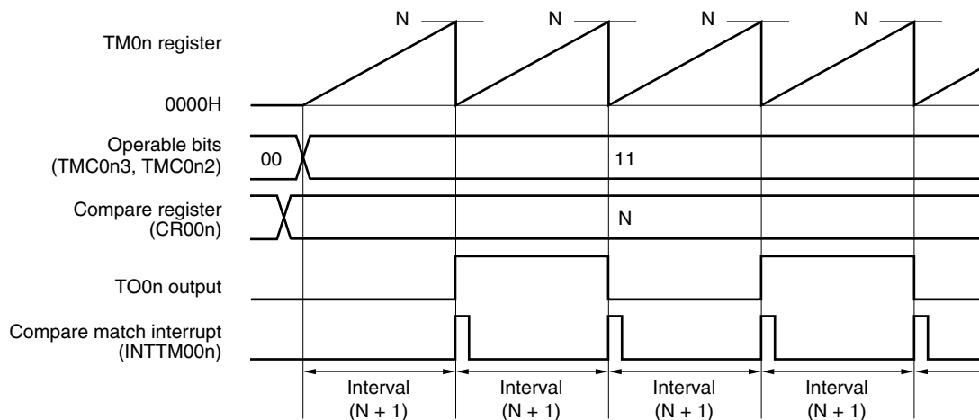
<R> Figure 7-21. Basic Timing Example of Square-Wave Output Operation
