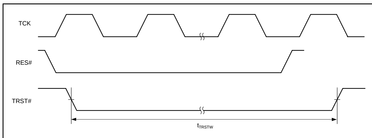
Figure 2.103 Boundary Scan TRST# Timing
