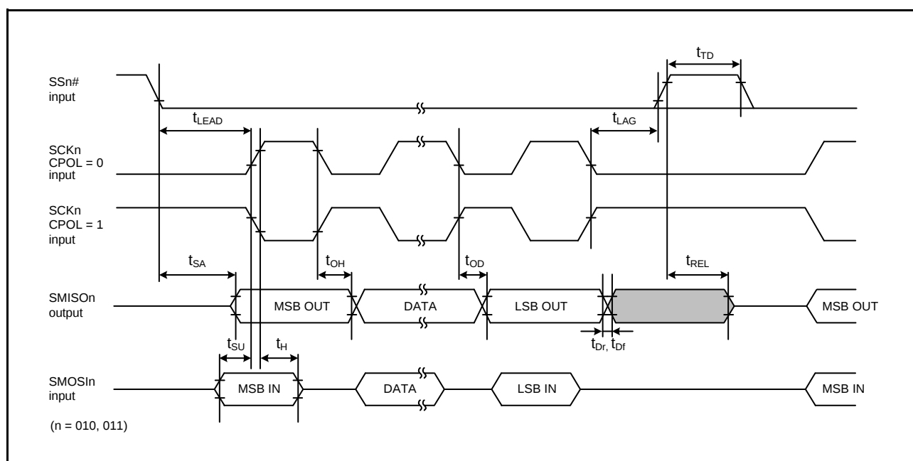
Figure 2.61 Simple SPI Timing (Slave, CPHA = 0)
