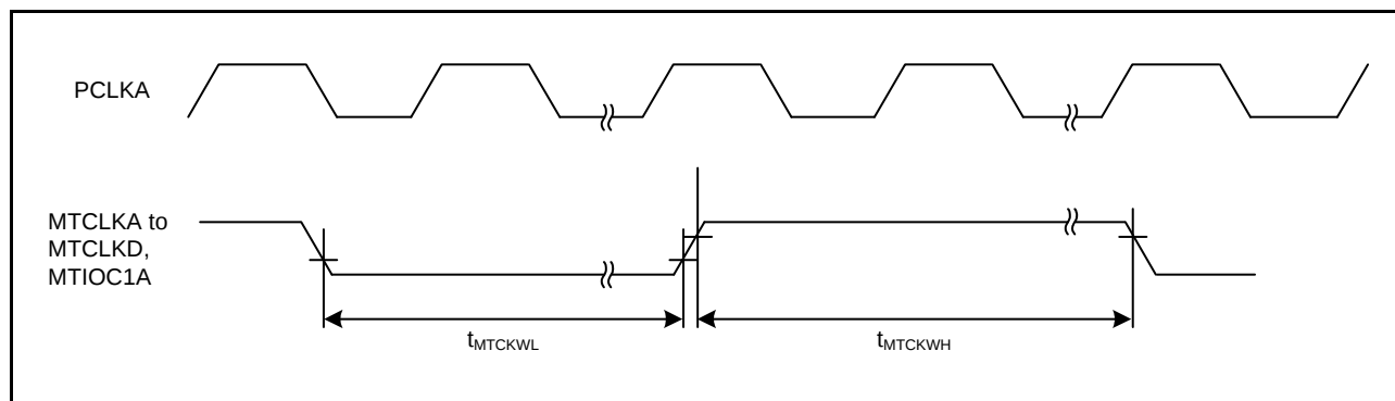
Figure 2.40 MTU Clock Input Timing
