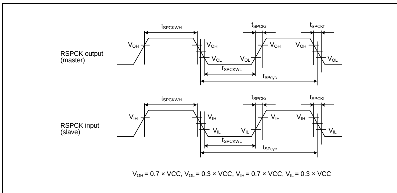
Figure 2.68 RSPCK Clock Timing
