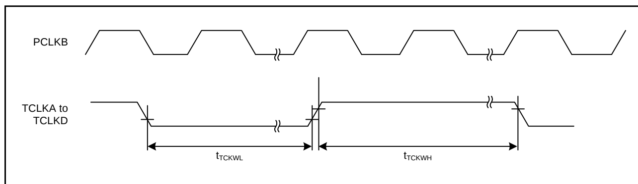
Figure 2.36 TPU Clock Input Timing
