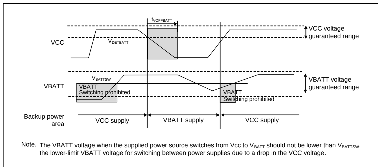
Figure 2.98 Battery Backup Function Characteristics
