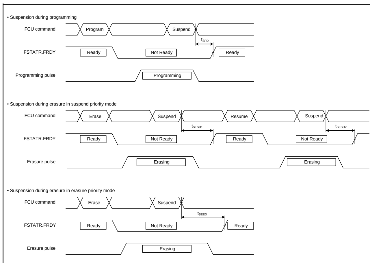
Figure 2.101 Flash Memory Programming/Erasure Suspension Timing
