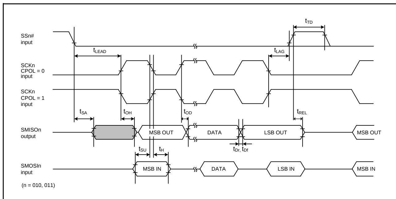
Figure 2.62 Simple SPI Timing (Slave, CPHA = 1)
