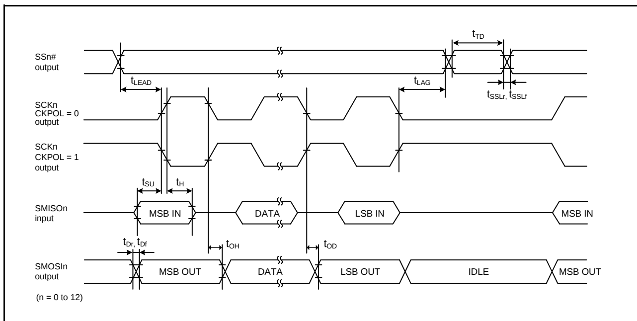
Figure 2.51 Simple SPI Timing (Master, CKPH = 1)
