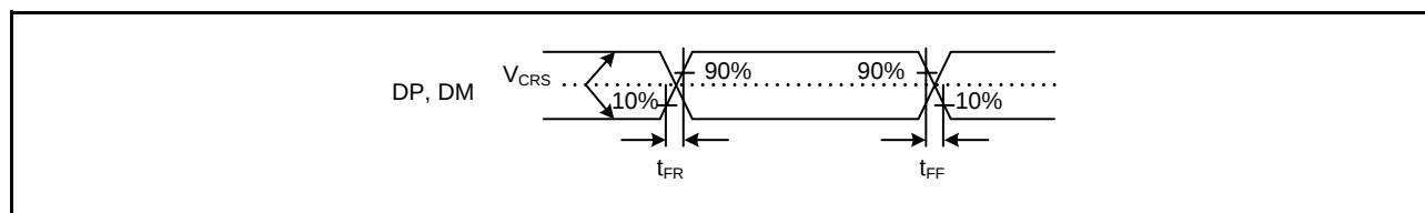
Figure 2.91 DP and DM Output Timing (Full-Speed)
