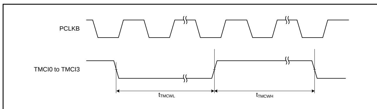
Figure 2.37 TMR Clock Input Timing
