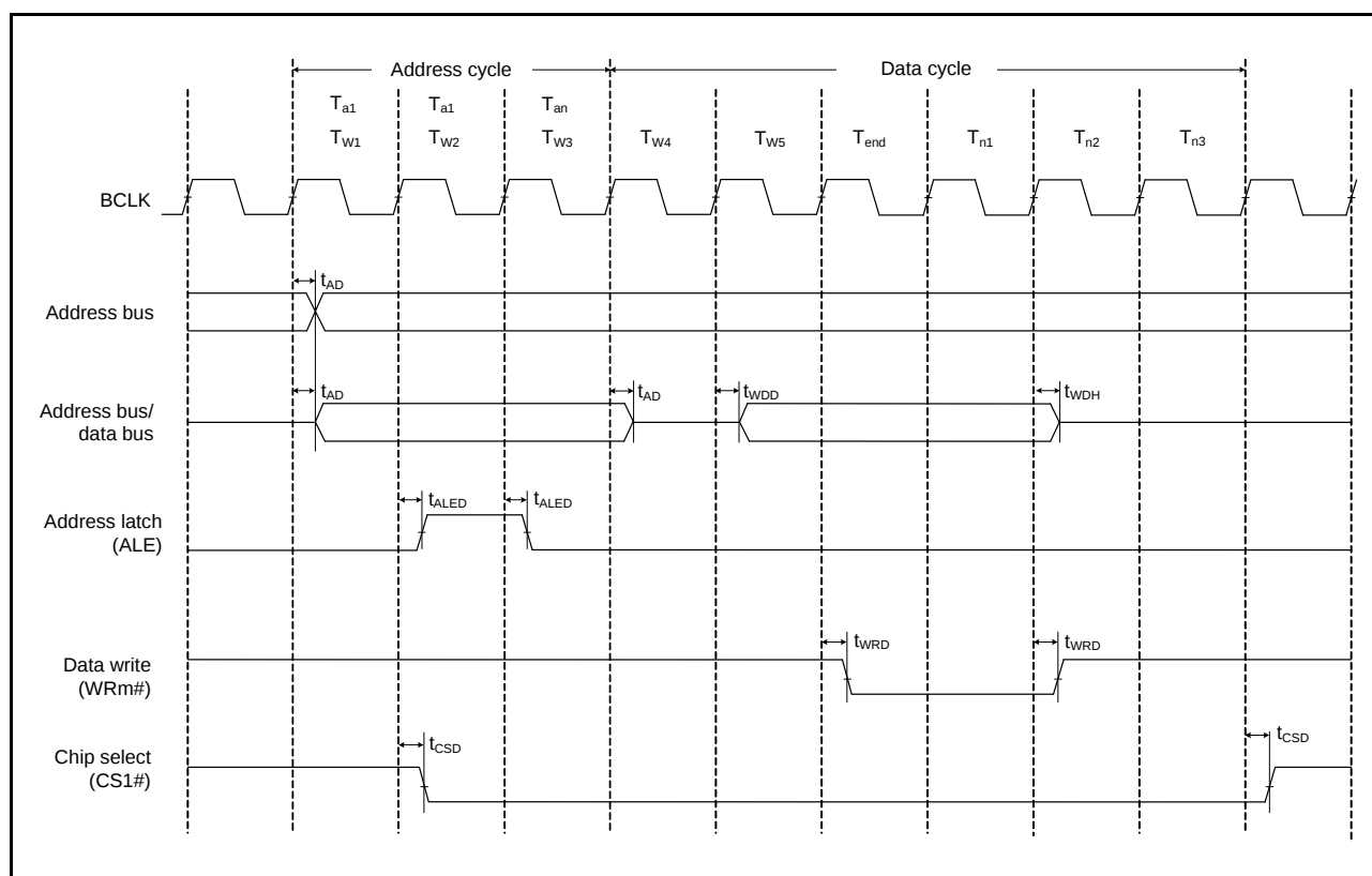
Figure 2.18 Address/Data Multiplexed Bus Write Access Timing
