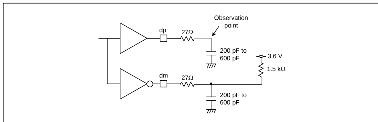
Figure 2.90 Test Circuit (Low Speed)
