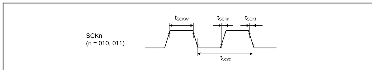
Figure 2.55 SCK Clock Input Timing
