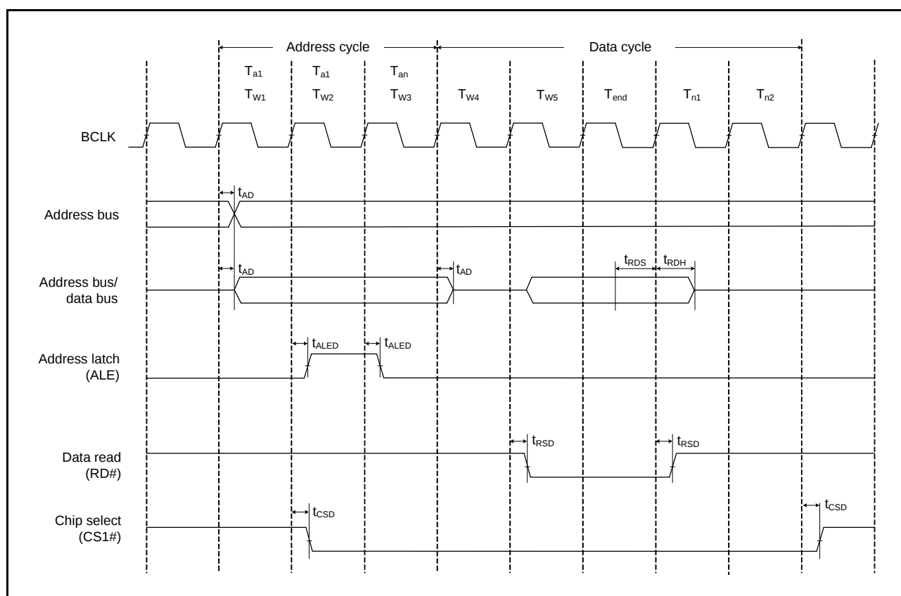
Figure 2.17 Address/Data Multiplexed Bus Read Access Timing
