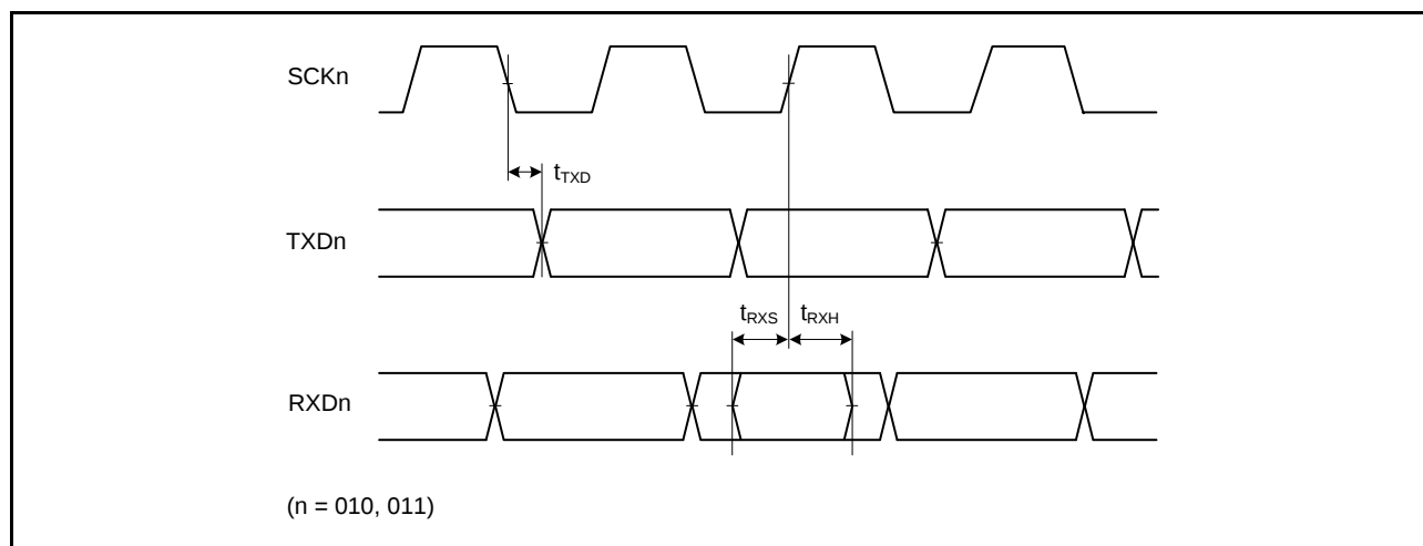
Figure 2.56 RSCI Input/Output Timing: Clock Synchronous Mode
