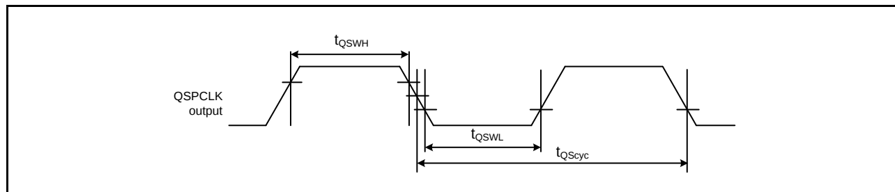
Figure 2.83 QSPIX Clock Timing
