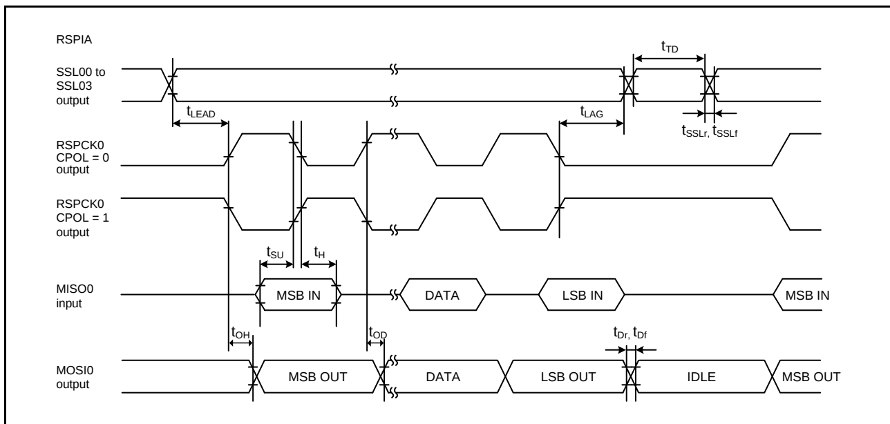
Figure 2.77 RSPIA Timing (Master, Motorola SPI, CPHA = 1)
