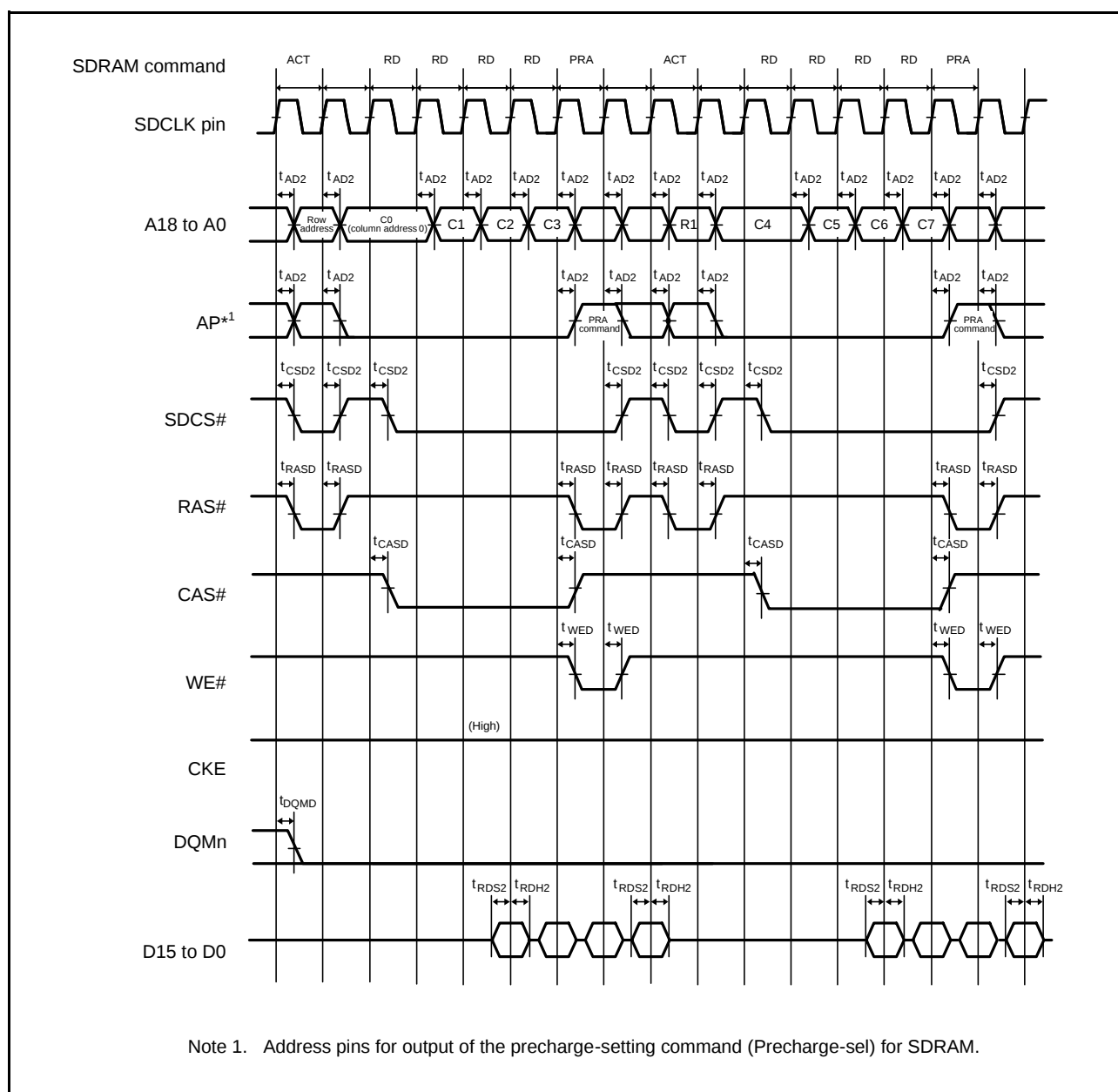
Figure 2.28 SDRAM Space Multiple Read Line Stride Bus Timing
