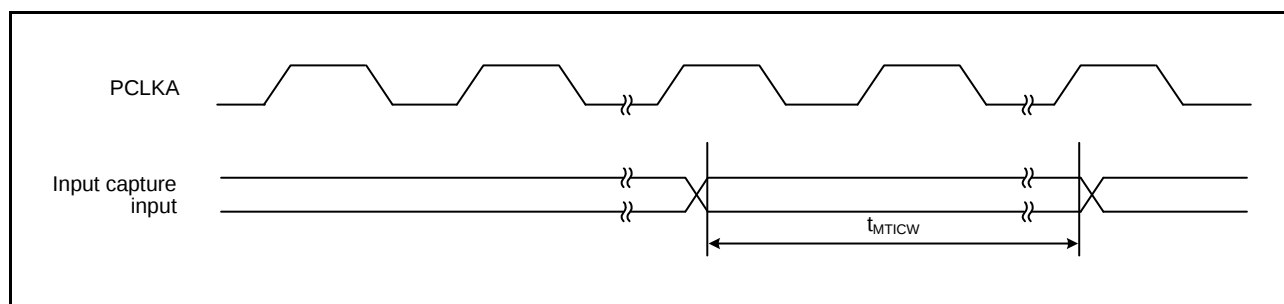
Figure 2.39 MTU Input Capture Input Timing
