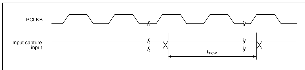
Figure 2.35 TPU Input Capture Input Timing
