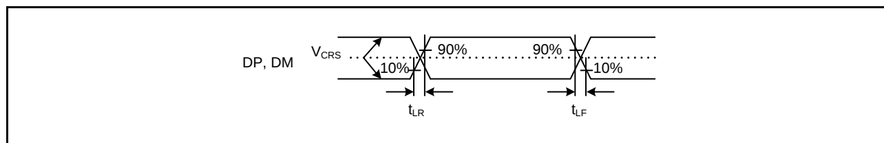
Figure 2.89 DP and DM Output Timing (Low Speed)
