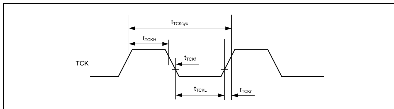
Figure 2.102 Boundary Scan TCK Timing
