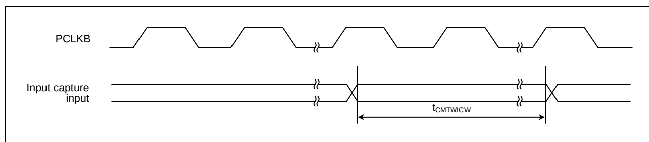
Figure 2.38 CMTW Input Capture Input Timing
