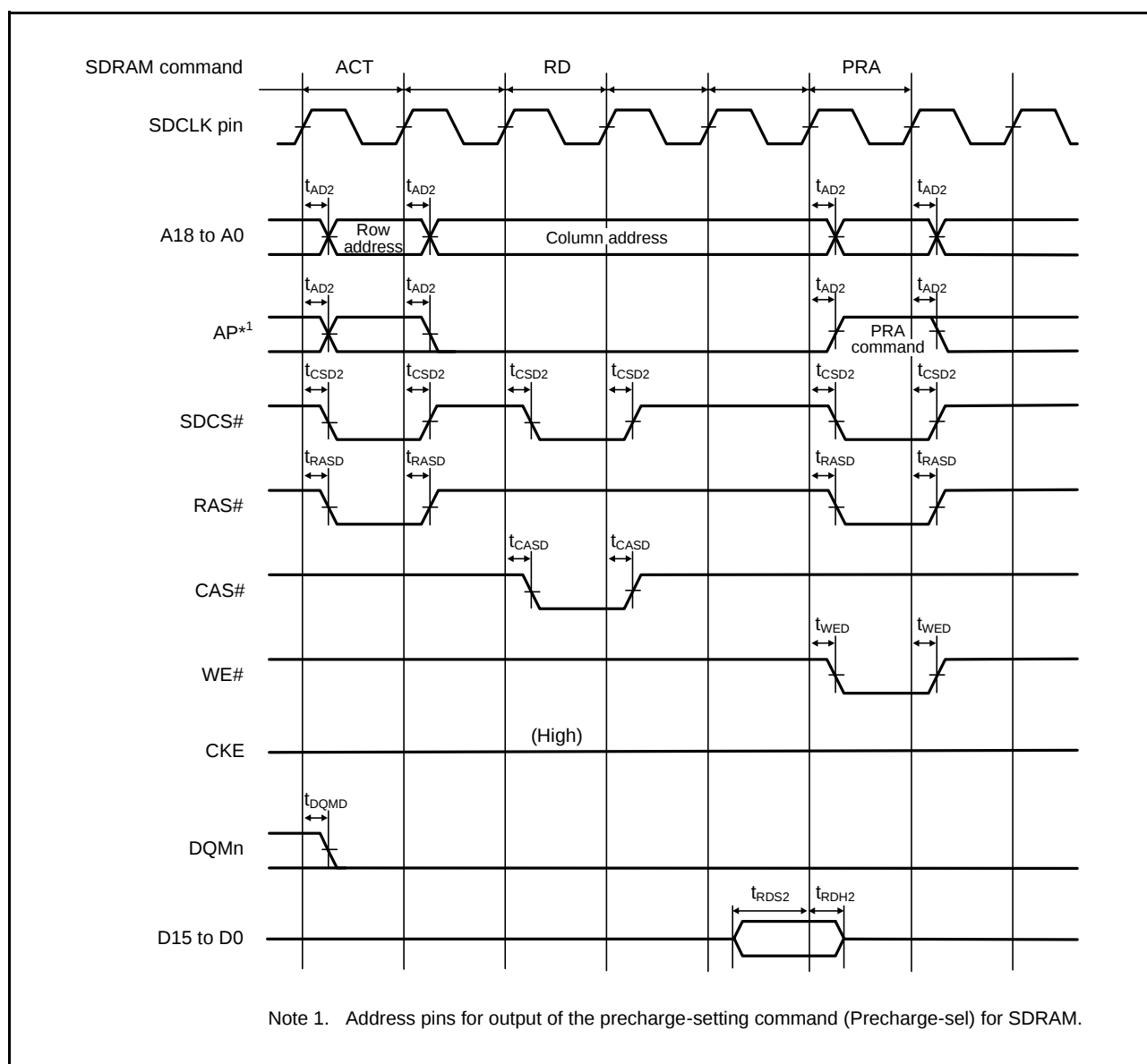
Figure 2.24 SDRAM Space Single Read Bus Timing
