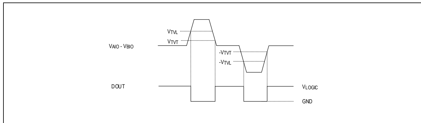
Figure 6. Receiver Threshold
