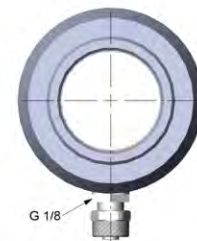
Mounting bracket (adjustable) for CTlaser
