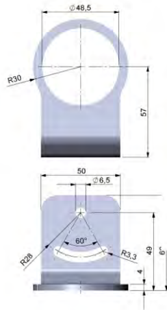
Mounting bracket (fixed) for CTlaser
