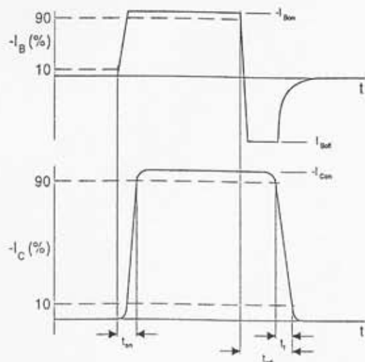
Fig. 1 Switching times waveforms.
