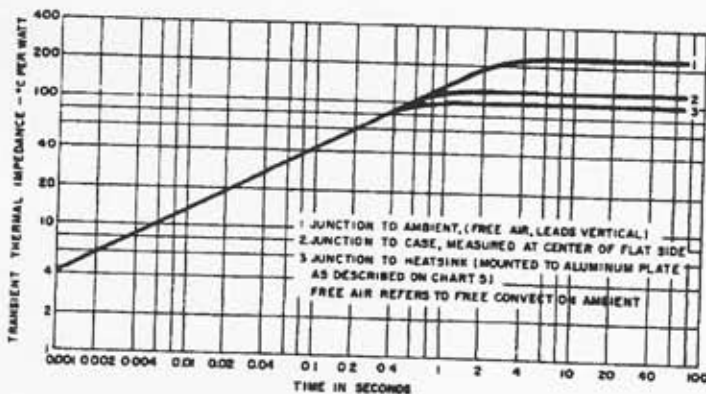
7. MAXIMUM TRANSIENT THERMAL IMPEDANCE
