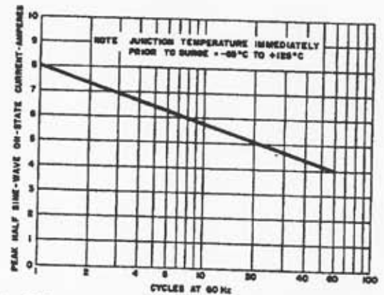
6. MAXIMUM ALLOWABLE SURGE (NON-REP) ON-STATE CURRENT
