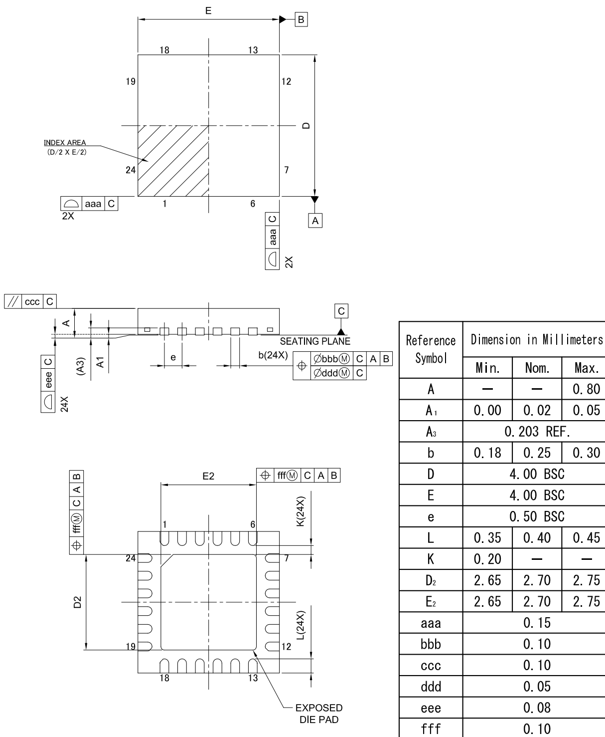
Figure 2.1 HWQFN 24-pin
