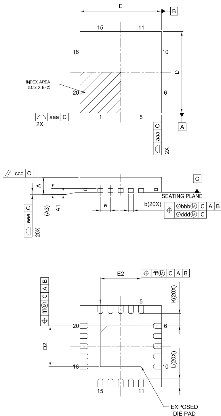
Figure 2.2 HWQFN 20-pin
