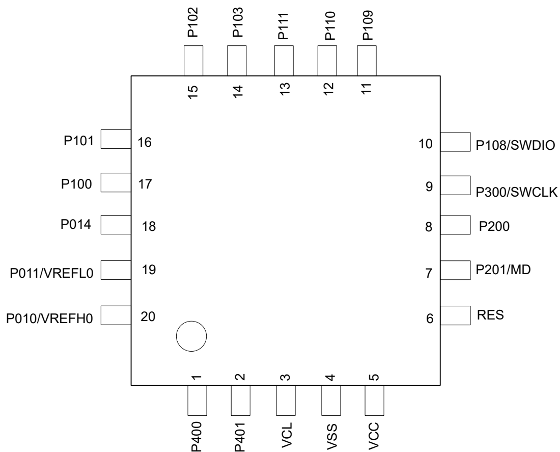
Figure 1.4 Pin assignment for HWQFN 20-pin (top view)
