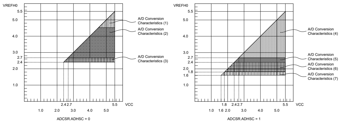
Figure 2.44 VCC to VREFH0 voltage range
