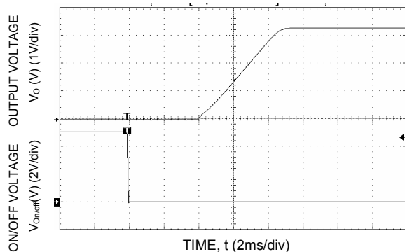
Figure 15. Typical Start-Up Using Remote On/Off with Low-ESR external capacitors ( 7 \times 150\ \mu\text{F} Polymer) ( V_{in} = 5.0\text{Vdc} , V_o = 3.3\text{Vdc} , I_o = 3\text{A} , C_o = 1050\ \mu\text{F} ).
