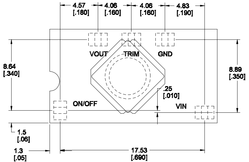
RECOMMENDED PAD LAYOUT PAD SIZE: MIN: 0.120" X 0.095" MAX: 0.135" X 0.110"
