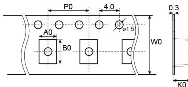
Figure 12 – Tape drawing (not to scale)
