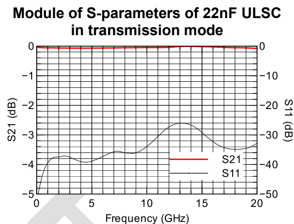
Figure 3 - 22nF ULSC Measured results (module of S-parameters)
