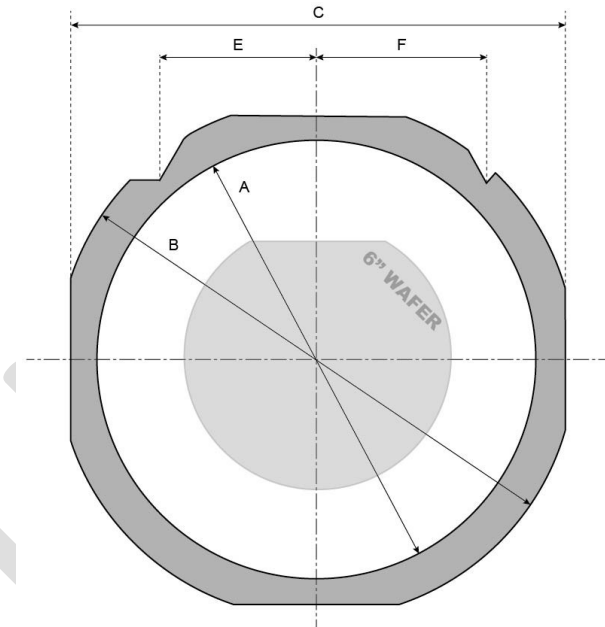
Figure 14 FF108 Frame with a 6 inch wafer
