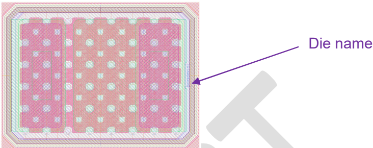
Figure 7 – Layout view
