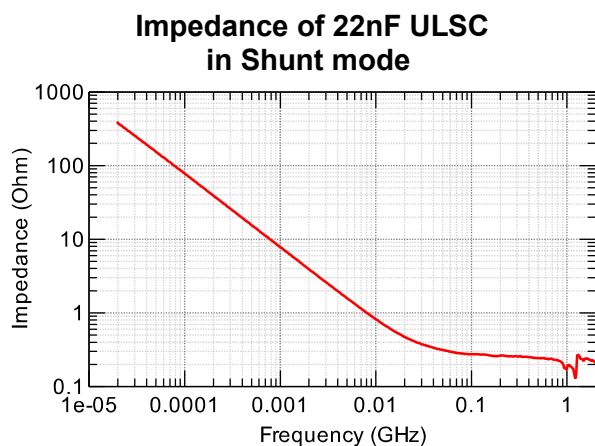
Figure 2 - 22nF ULSC Measured results (module of Z-parameters)
