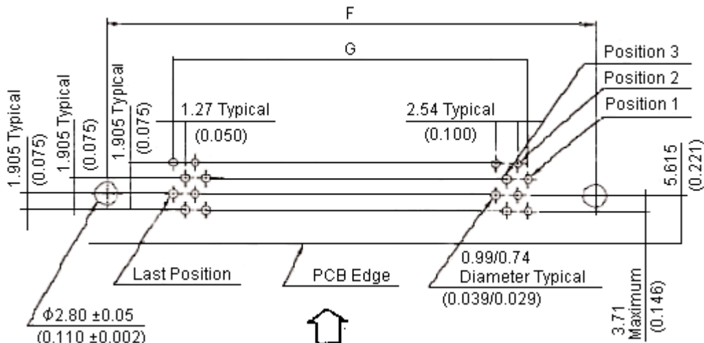
Connector Mating Side Recommended PCB Hole Pattern
