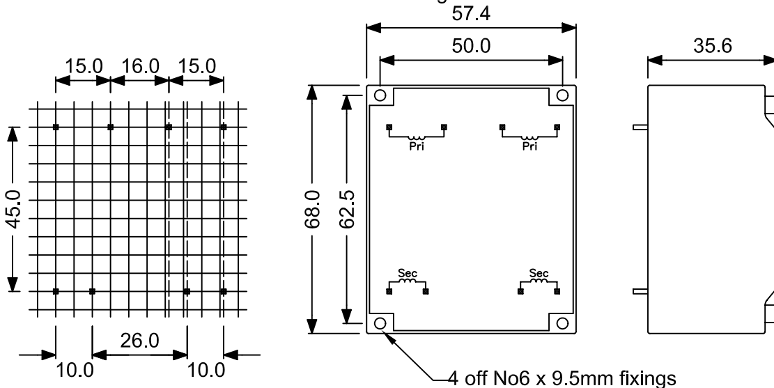
Outline Drawing
