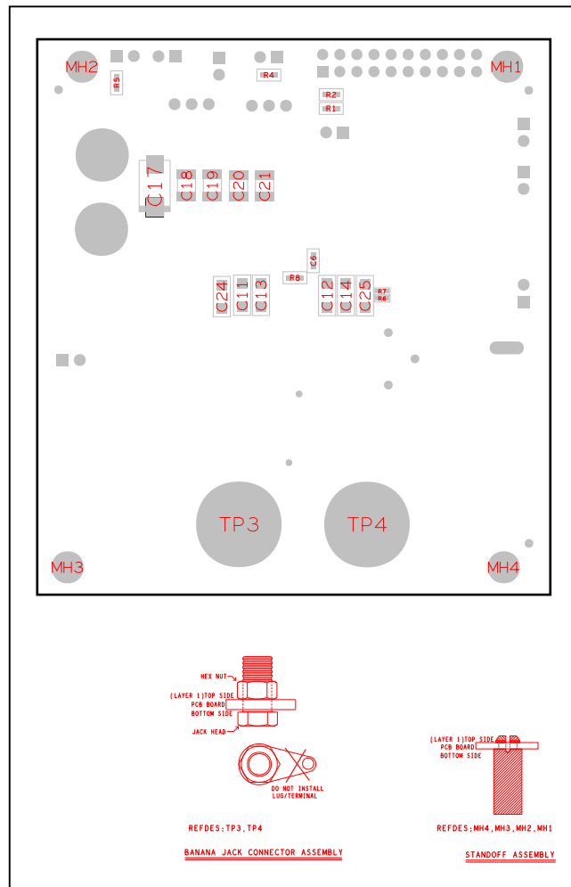
Figure 11. MAX20011C EV Kit PCB Layout—Bottom Assembly
