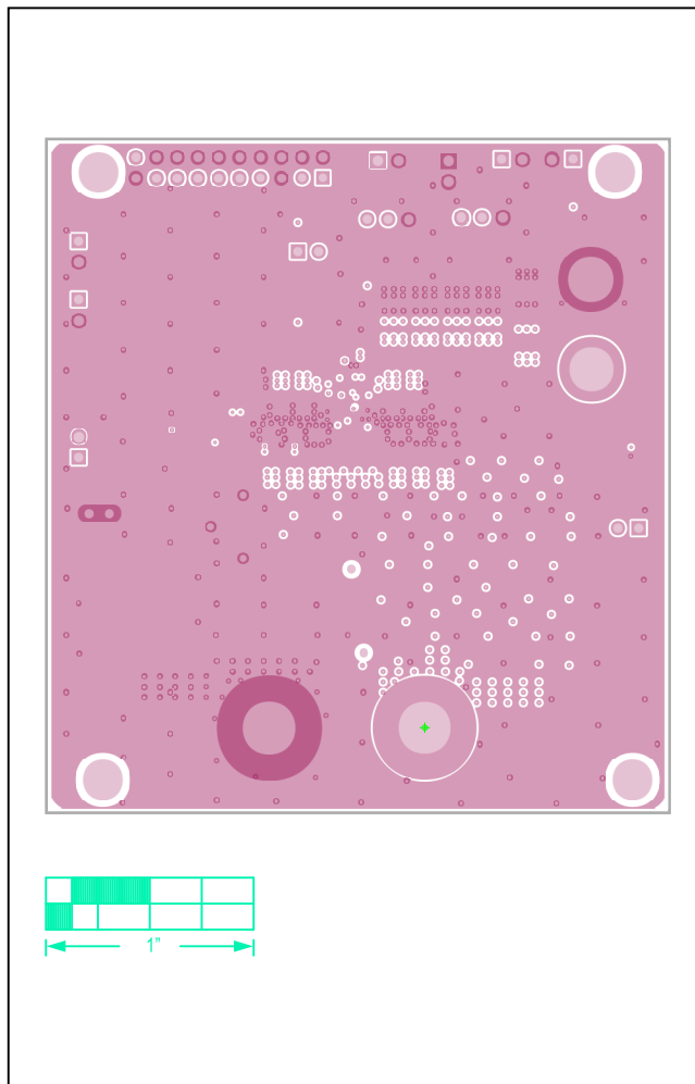
Figure 5. MAX20011C EV Kit PCB Layout—Inner Layer 3
