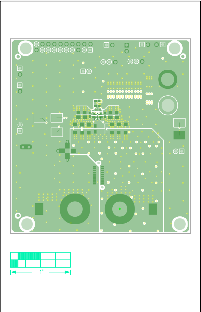
Figure 3. MAX20011C EV Kit PCB Layout—Top Layer
