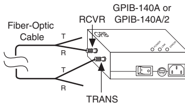
Figure 2-3. GPIB Extender Self-Test Configuration
