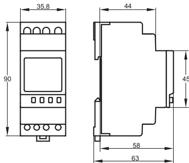
SC 18.10 pro (1 channel)
