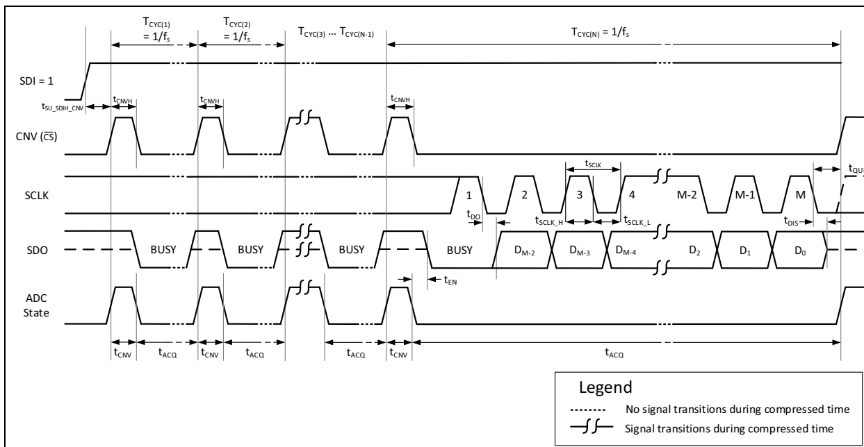
FIGURE 6-8: Timing Diagram for Accumulator Operation in 3-Wire CS Mode with BUSY Status Indicator Output Bit.
