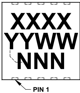
10-Lead TDFN (3 × 3 × 0.8 mm)
