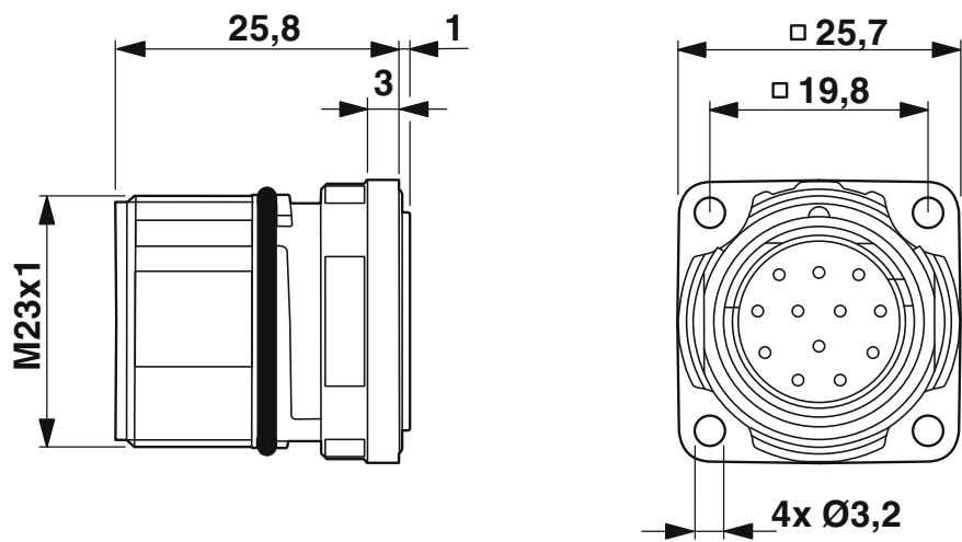
Dimensional drawing
