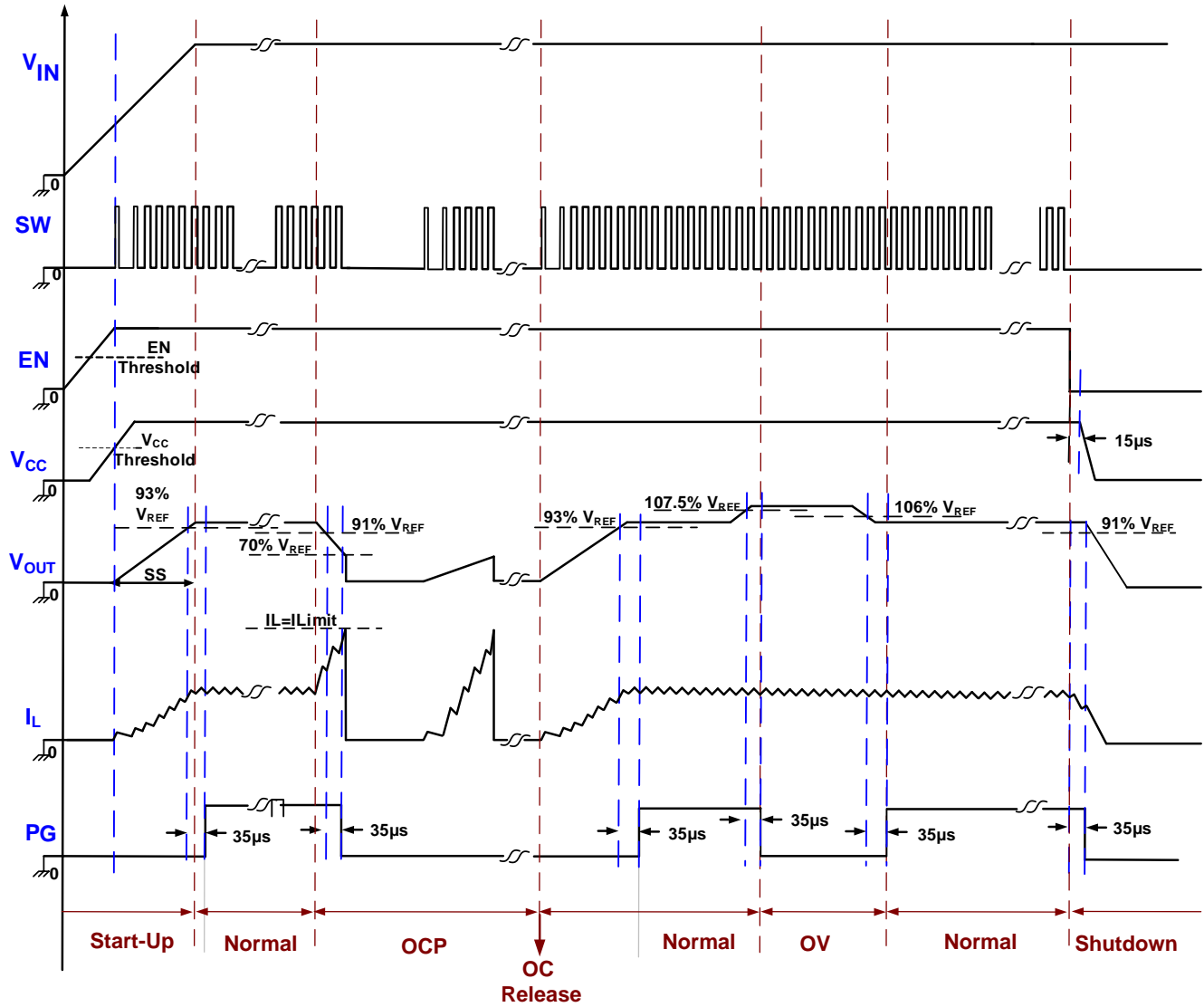
Figure 2: Timing Sequence
