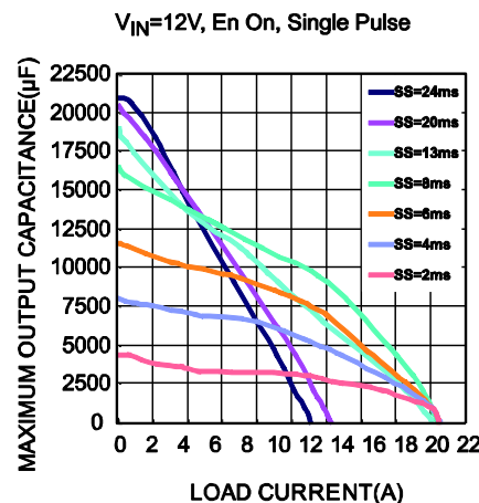
Maximum Output Cap. vs. Load Current V_{IN}=12V , En On, Single Pulse
