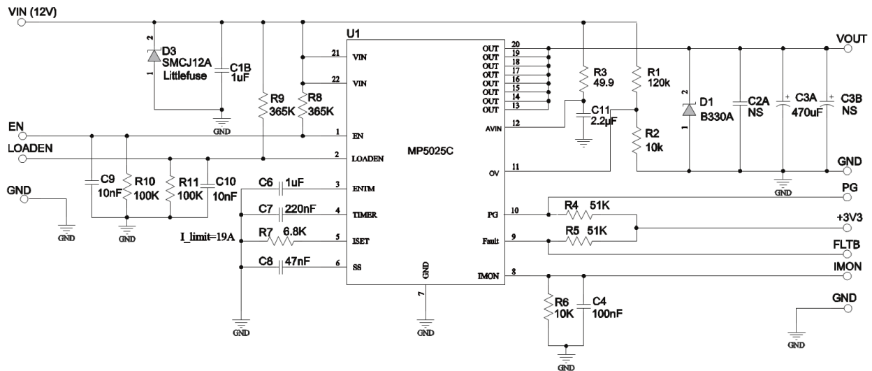
Figure 11: Over-Current Limit ≥7A Applications
