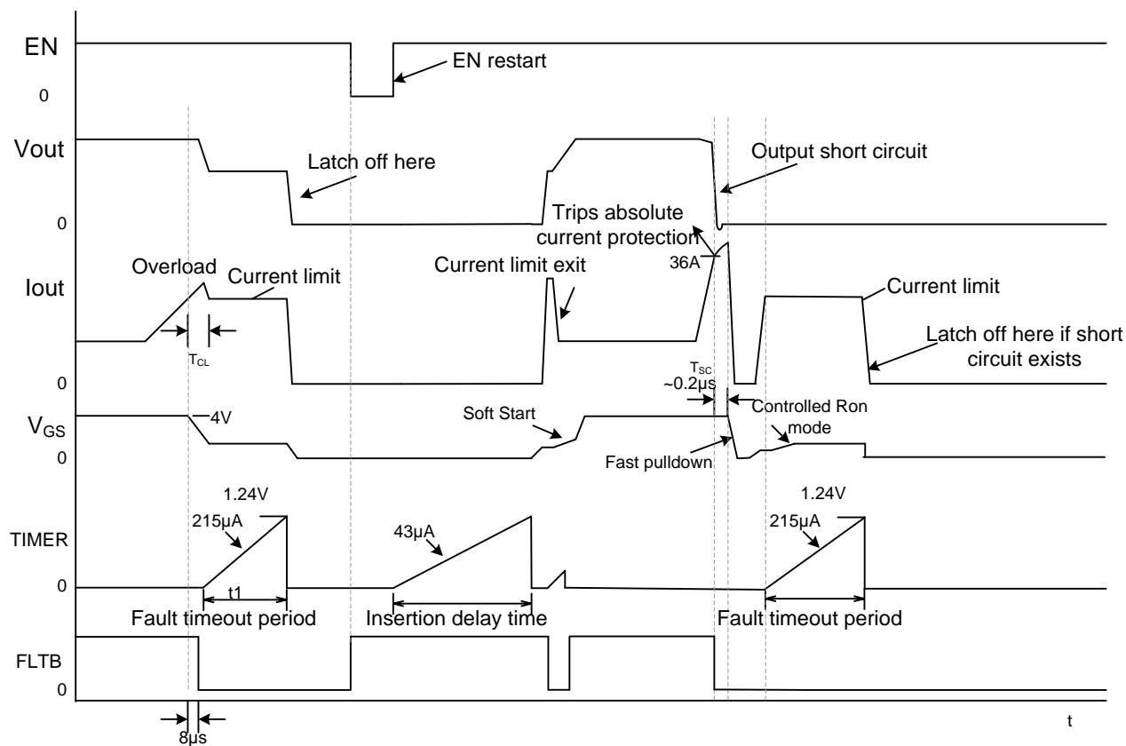
Figure 2: Over-Current Protection
