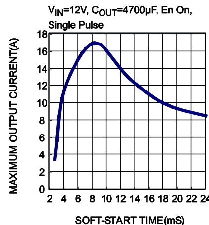
Maximum Output Current vs. Soft Start Time V_{IN}=12V , C_{OUT}=4700\mu F , En On, Single Pulse
