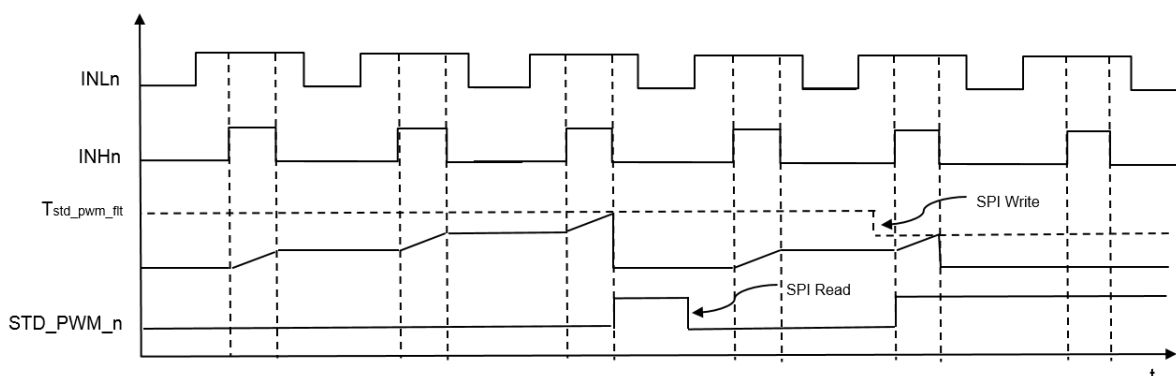
Figure 41. Shoot-Through diagnosis on PWM inputs: functional operation
