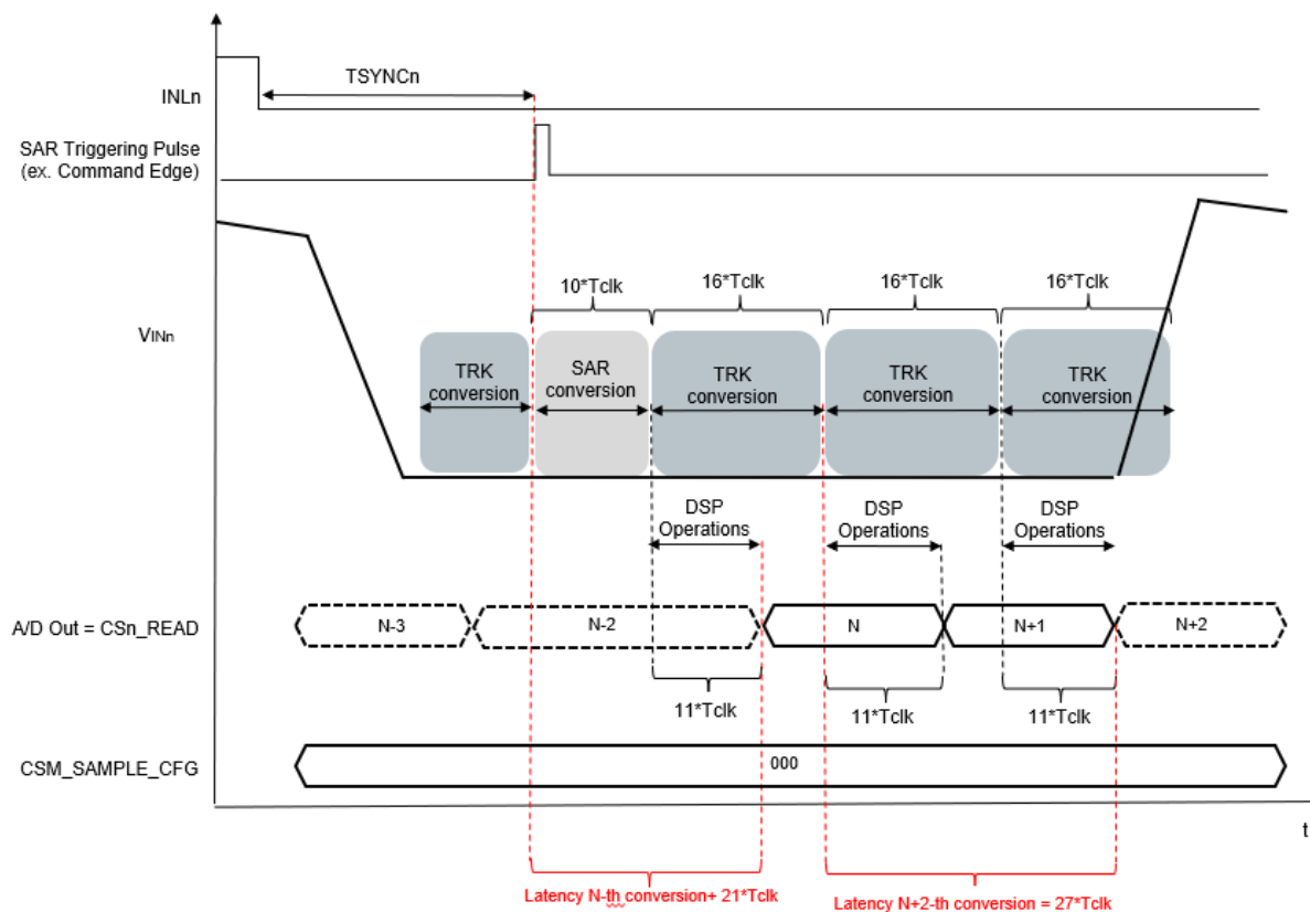
Figure 56. Free running sampling timing diagram - zero current (offset) + command edge-triggering
