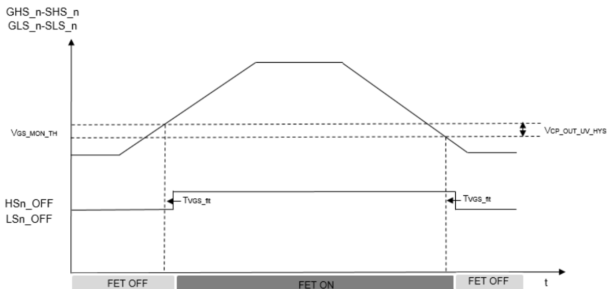
Figure 38. VGS Monitor operative ranges
