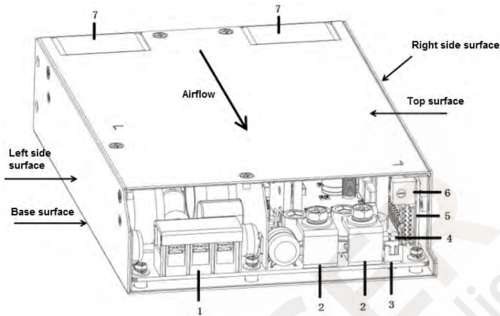
Fig. 1: Appearance information of TGR1000-xx
