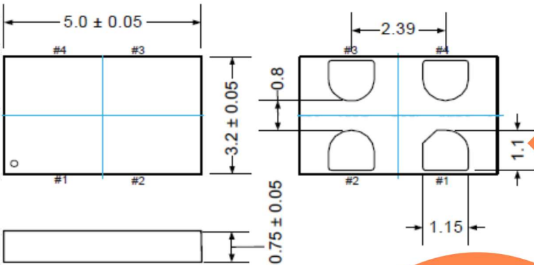
5.0 x 3.2mm Package (Option “FL”)
