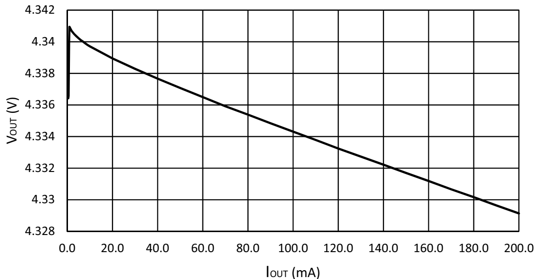
Figure 99. SLG46580 LDO Load Regulation, HIGH POWER Mode, T = 25^{\circ}\text{C} , V_{DD} = 5\text{V} , V_{OUT} = 4.35\text{V}
