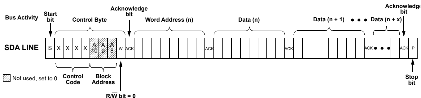
Figure 89. Sequential Write Command, \overline{R/W} = 0
