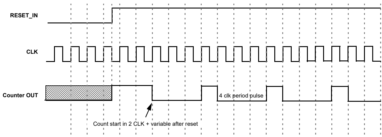
Figure 28. Counter Mode Timing with Reset Signal (only for DLY/CNT0)
