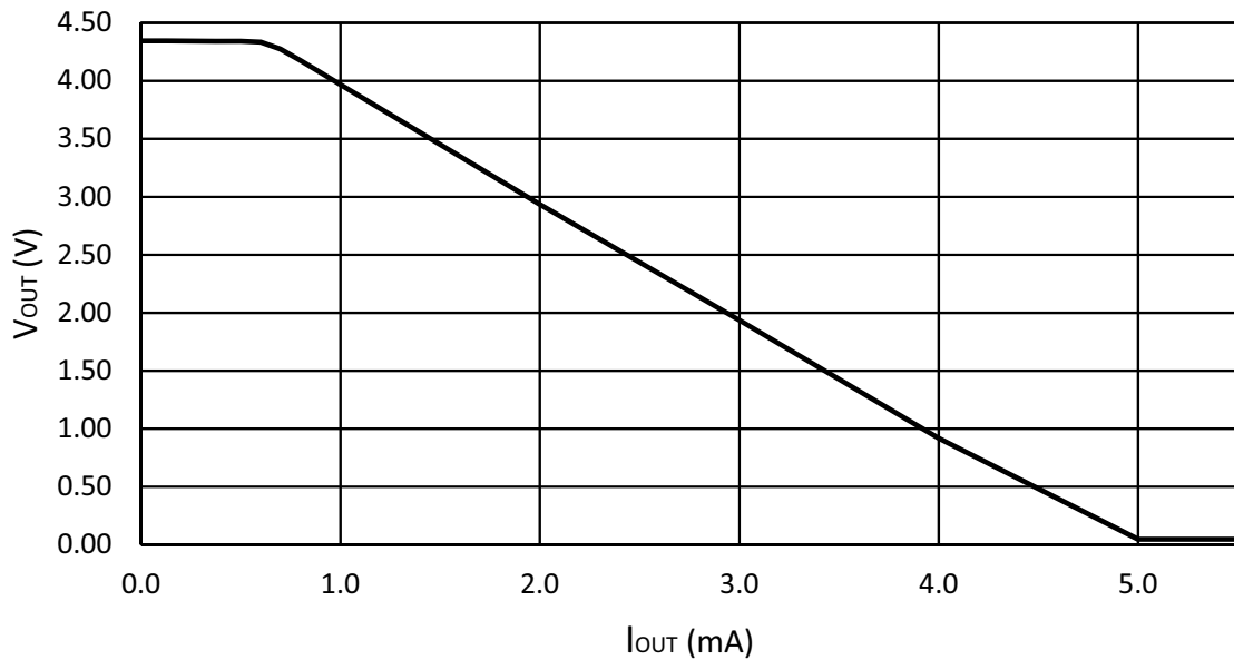
Figure 100. SLG46580 LDO Load Regulation, LOW POWER Mode, T = 25^{\circ}\text{C} , V_{DD} = 5\text{V} , V_{OUT} = 4.35\text{V}
