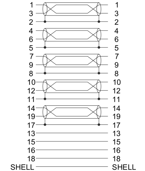
PIN Assignment P1 HDMI AM P2 HDMI AM
