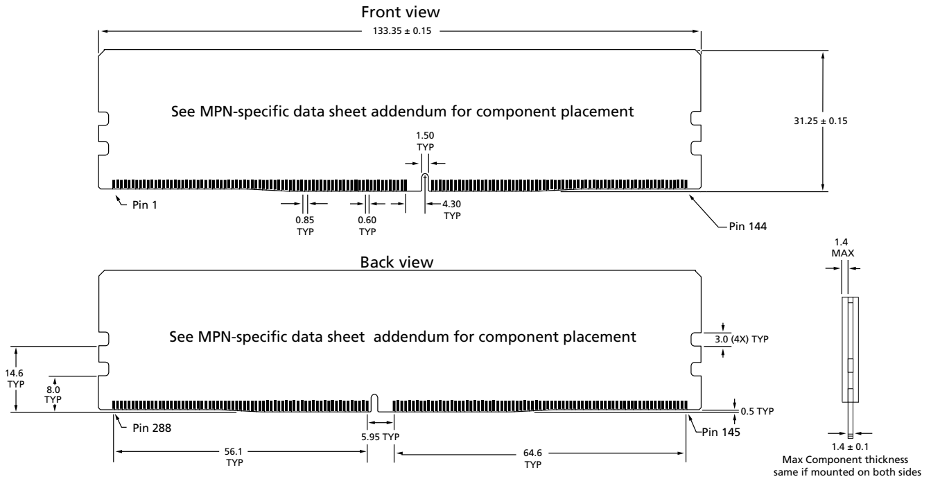
Figure 1: 288-Pin DDR4 LRDIMM
