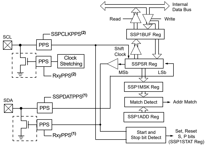
FIGURE 32-3: MSSP BLOCK DIAGRAM (I 2 C CLIENT MODE)
