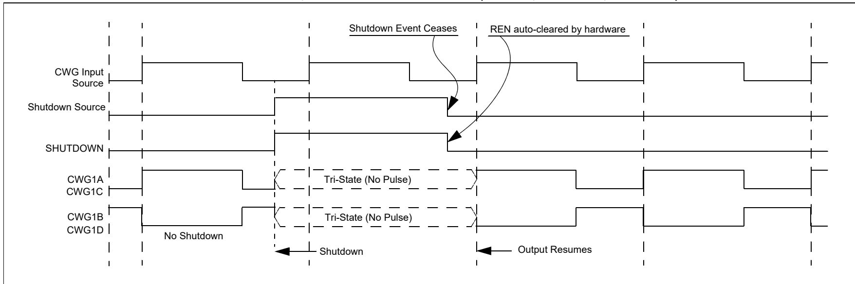
FIGURE 30-14: SHUTDOWN FUNCTIONALITY, AUTO-RESTART ENABLED (REN = 1, LSAC = 01, LSB D = 01)
