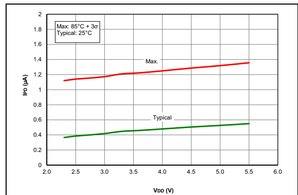
FIGURE 38-24: IPD Base, VREGPM = 1, PIC16F15313/23 Only.
