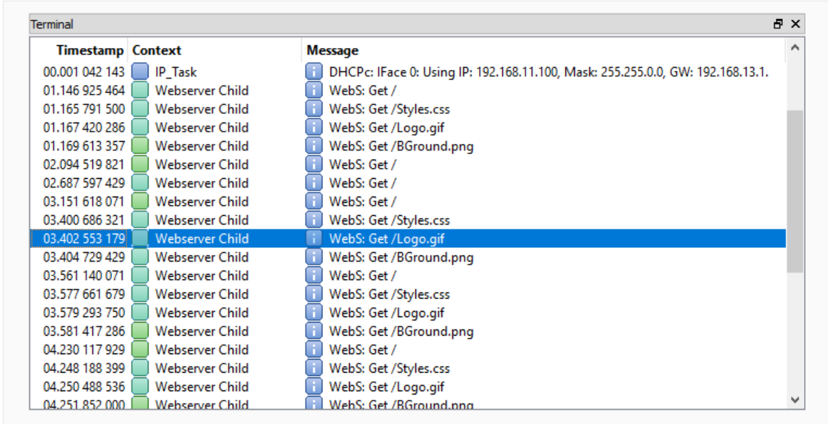
SystemView Terminal
