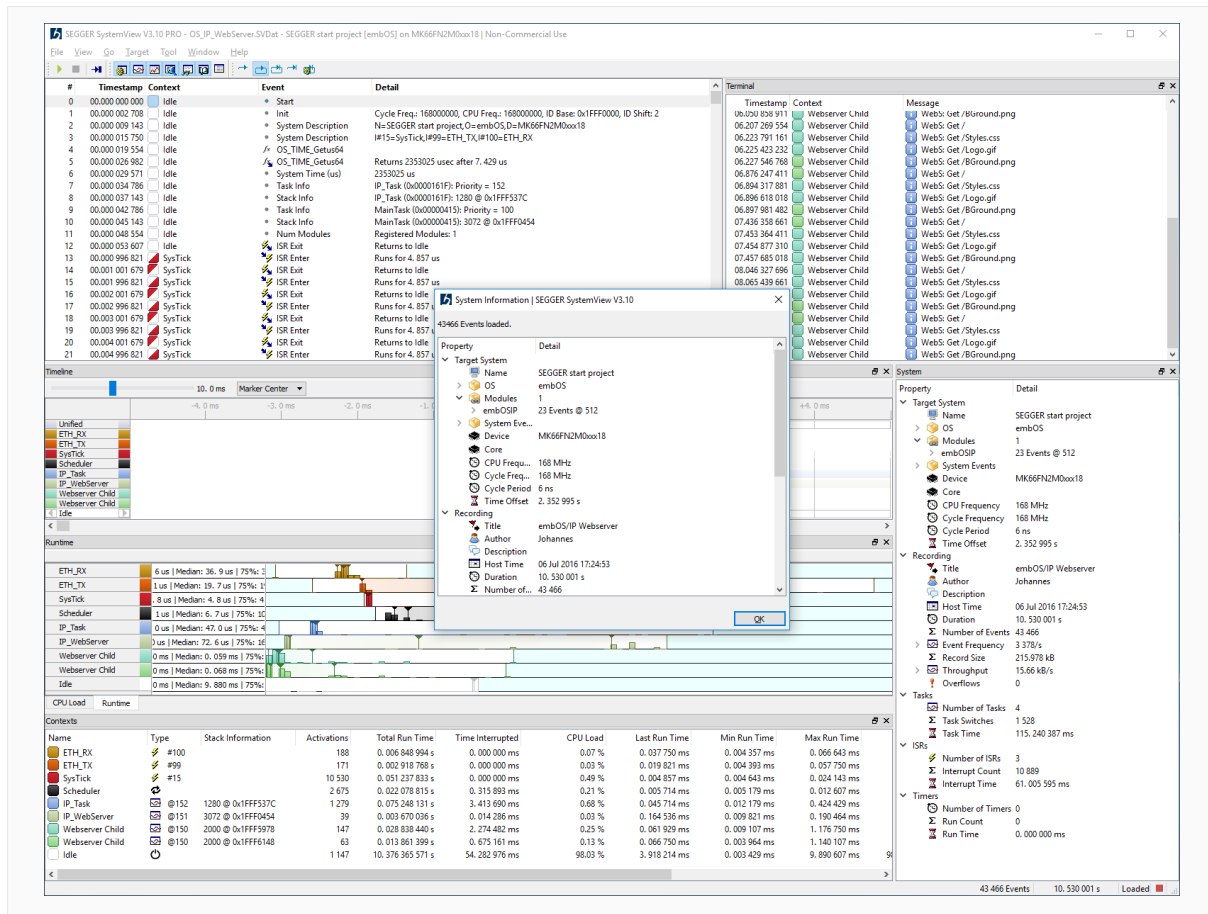
SystemView after File Load
