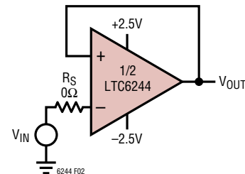
Figure 2. Unity Gain Follower Test Circuit
