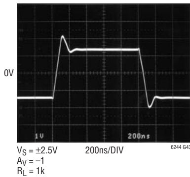
Large-Signal Response
