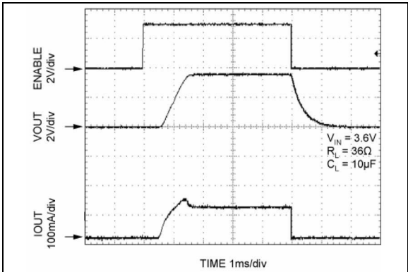
FIGURE 2-23: Turn-On/Turn-Off Timing.
