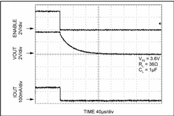
FIGURE 2-22: Turn-On/Turn-Off Timing.
