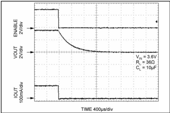
FIGURE 2-24: Turn-On/Turn-Off Timing.
