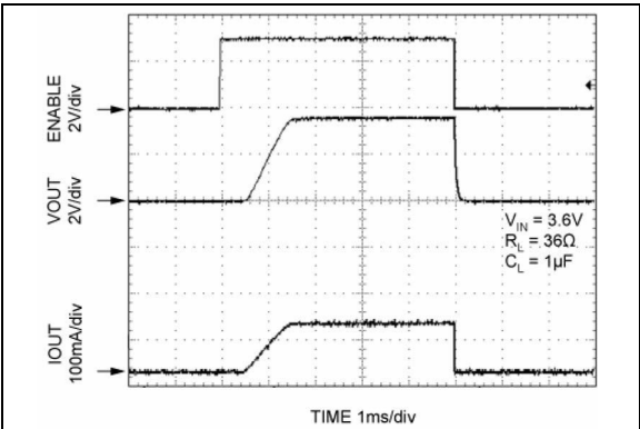
FIGURE 2-21: Turn-On/Turn-Off Timing.
