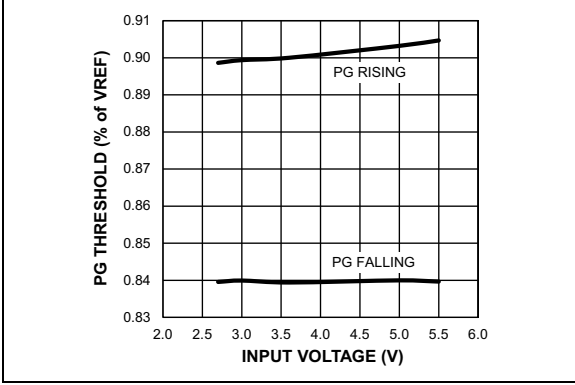
FIGURE 2-11: Power Good Thresholds vs. Input Voltage.
