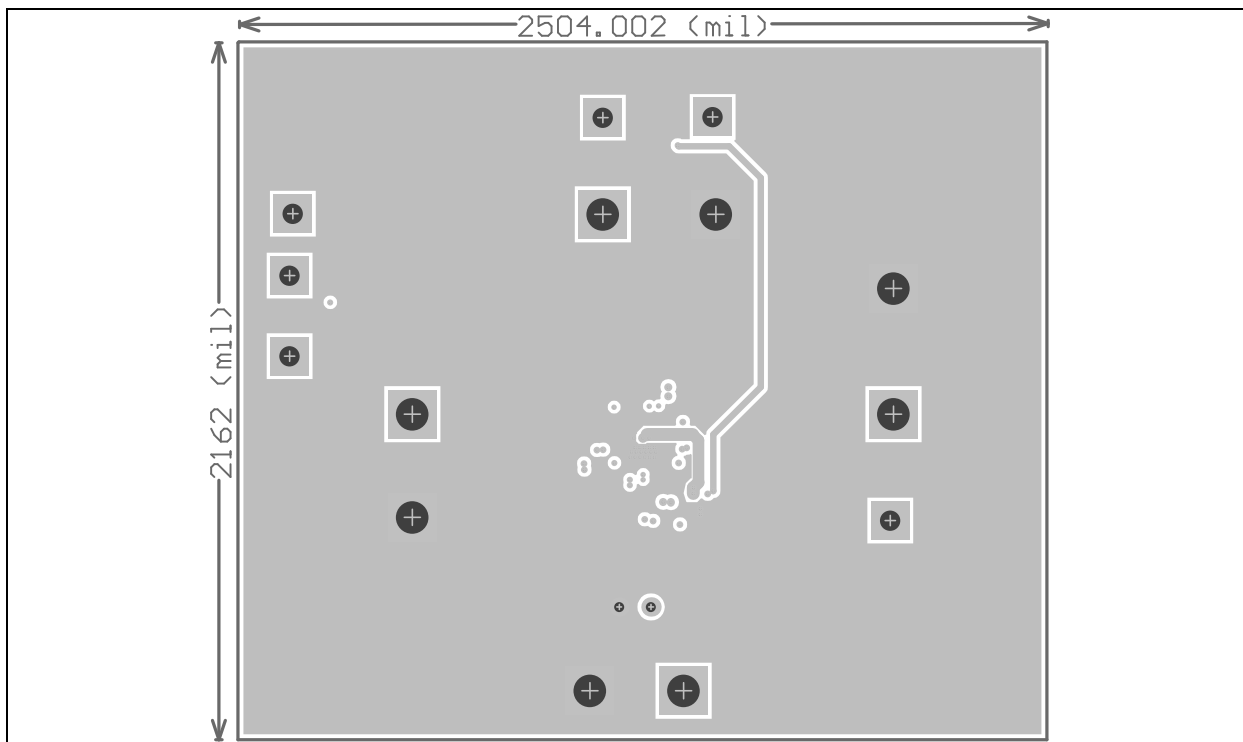
FIGURE 7-3: Mid Layer 2.
