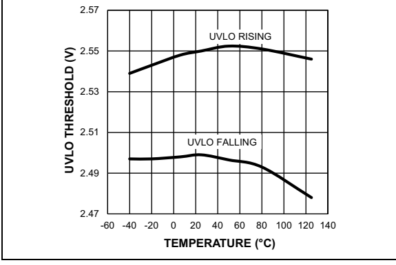
FIGURE 2-12: UVLO Threshold vs. Temperature.
