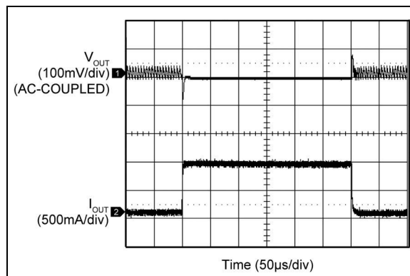
FIGURE 2-28: Load Transient (50 mA to 1A).
