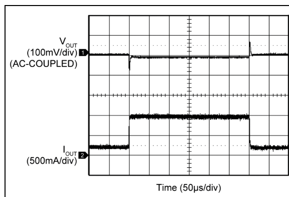
FIGURE 2-29: Load Transient (200 mA to 1A).
