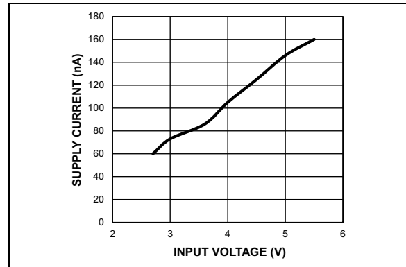
FIGURE 2-4: Shutdown Current vs. Input Voltage.
