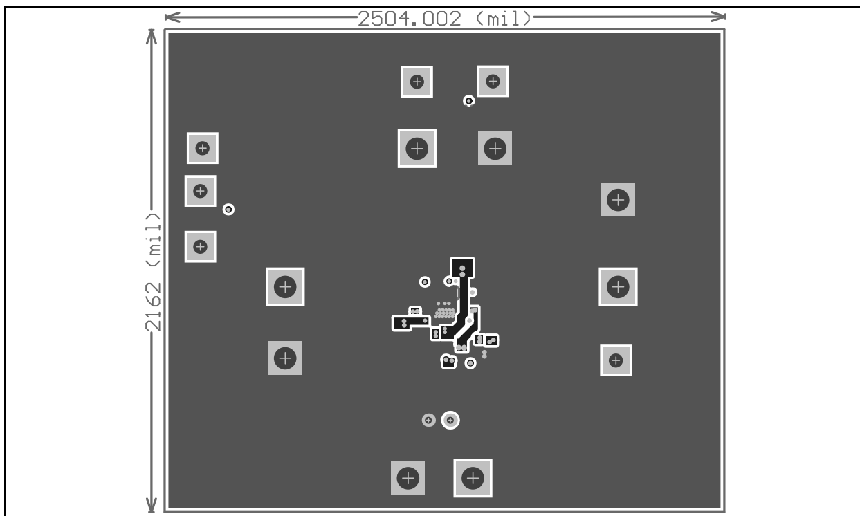
FIGURE 7-4: Bottom Layer.
