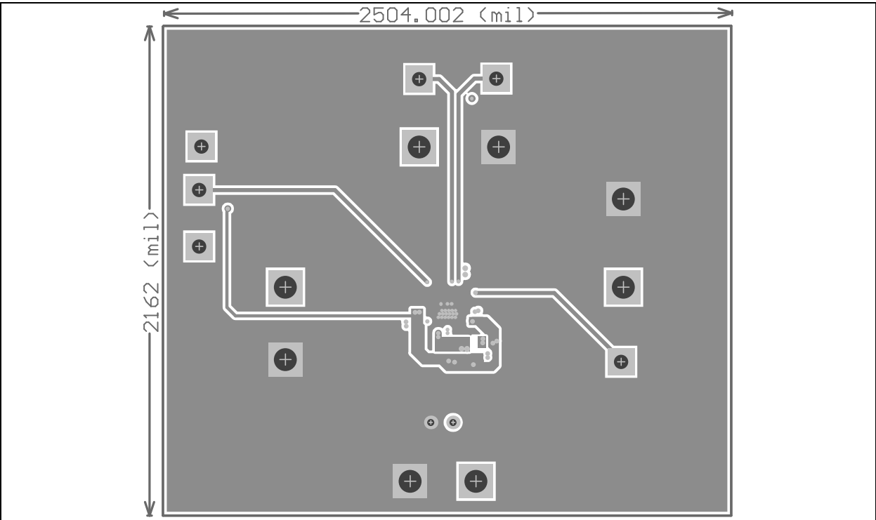
FIGURE 7-2: Mid Layer 1.
