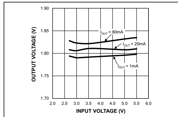
FIGURE 2-5: Line Regulation (Low Loads).
