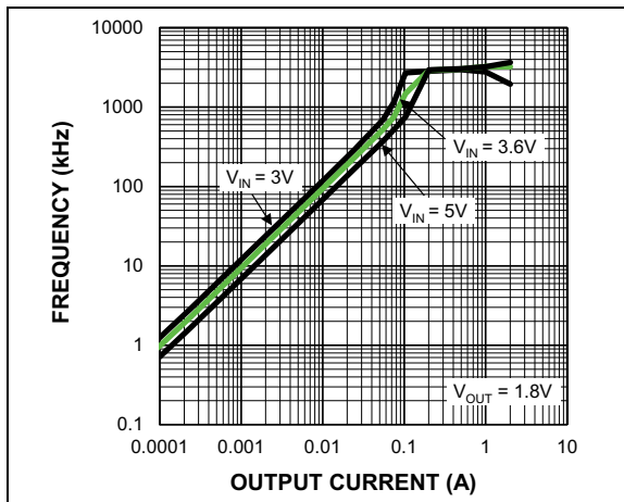
FIGURE 5-3: Switching Frequency vs. Output Current.
