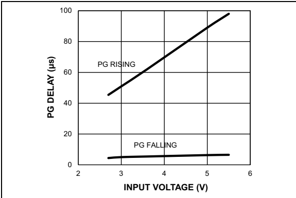
FIGURE 2-10: Power Good Delay Time vs. Input Voltage.
