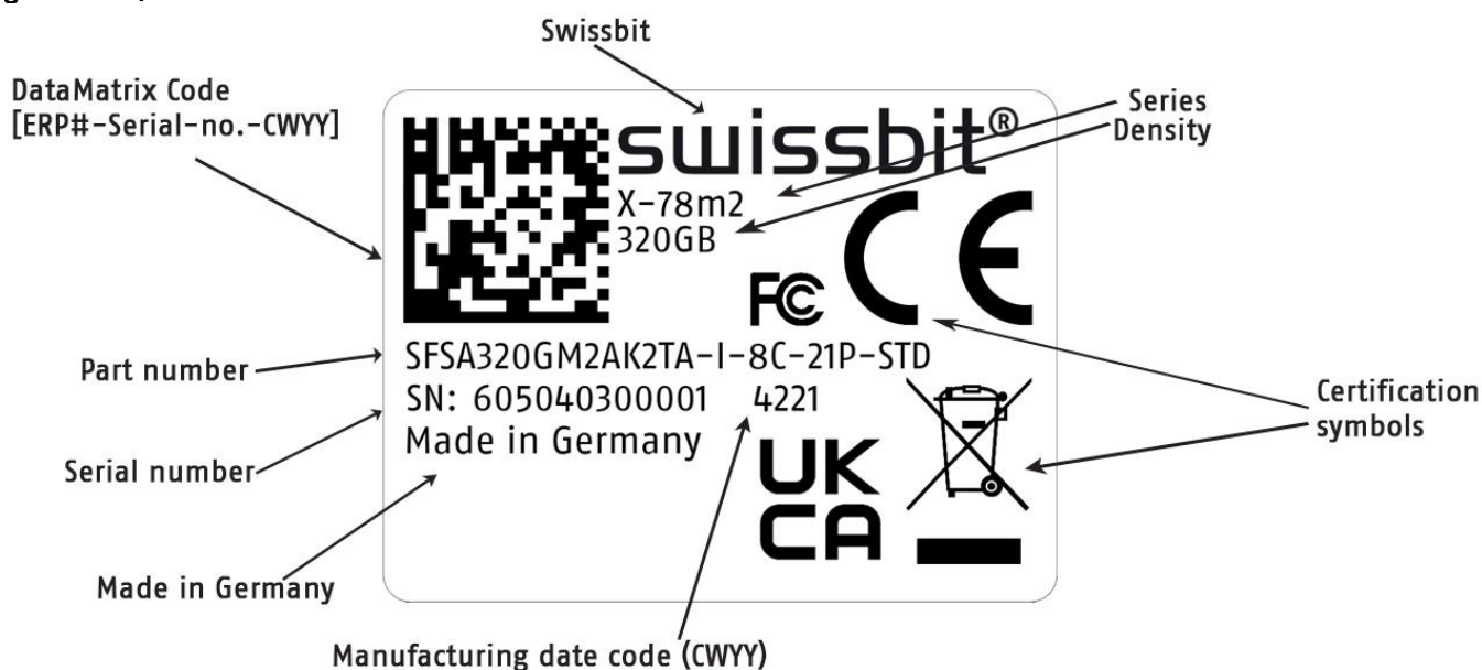
Figure 6: X-78m2 label details
