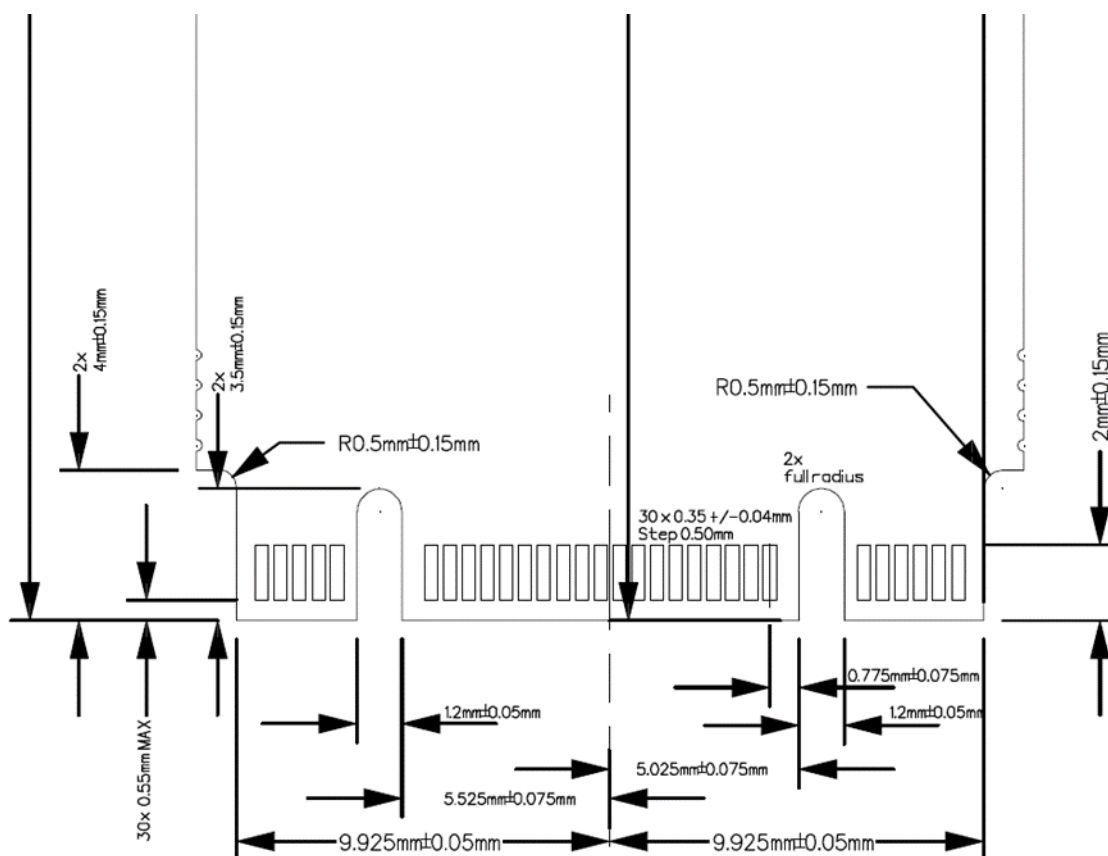
Figure 4: M.2 Connector Dimensions in mm
