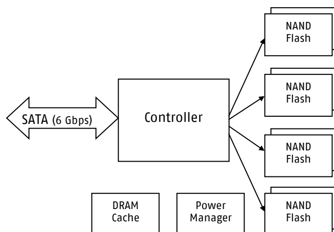
Figure 1: X-78m2 SATA Functional Block Diagram
