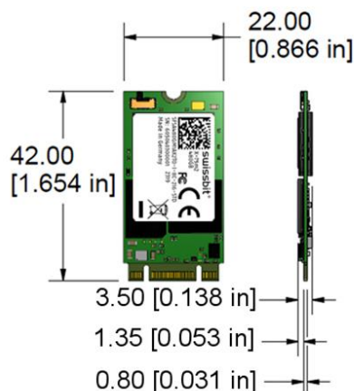
Figure 3: X-78m2 SATA SSD Dimensions in mm [in]
