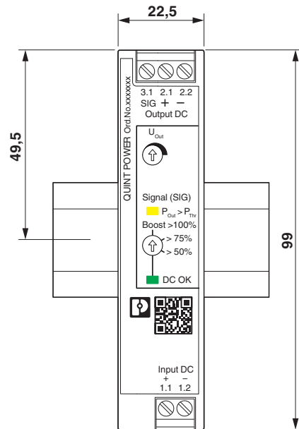
Figure 4 Device dimensions (dimensions in mm)
