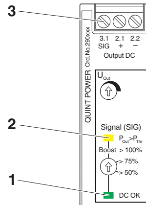
Figure 19 Position of signaling elements
