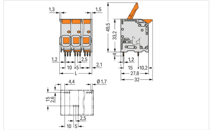
Dimensions in mm L = (pole no. - 1) x pin spacing + 12.8 mm
